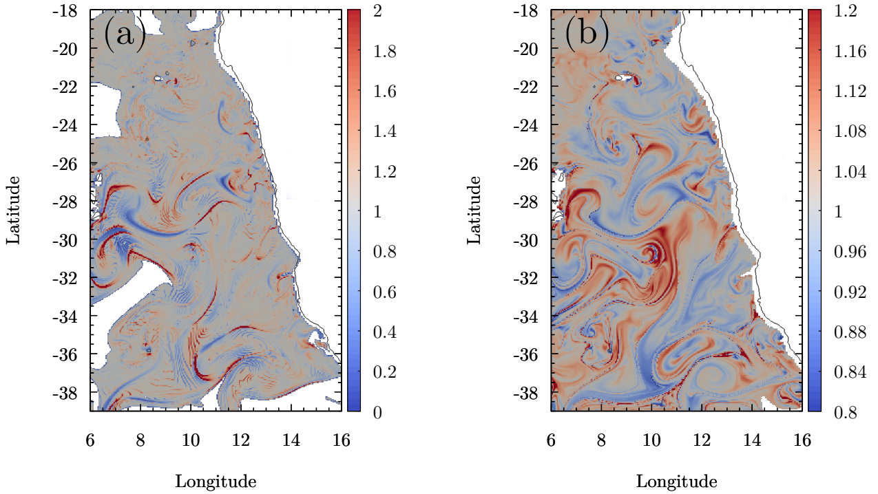
Figure 7. Results of the clustering numerical experiments of Sect. 5. (a) N_f/N_0 , the number of particles N_f arriving to an horizontal box of size 1/25^\circ in the horizontal layer at z = -1000 m, normalized by the number of particles N_0 = 1000 released from the upper z = -100 m layer. (b) The corrected dilation factor \delta(\mathbf{x}, t_f)^{-1} \cos(\theta_f)/\cos(\theta_0) mapped on the final z = -1000 m layer. It gives the ratio between horizontal densities at the final and initial locations, corrected with the latitudinal dependence of the horizontal boxes used in panel (a), to give an estimation of the local particle number ratio between lower and upper layer. Black thin line represents the coastline; white oceanic areas indicate in (a) regions which do not receive any falling particles; in (b) regions from which the backward integration ends up outside the domain.
