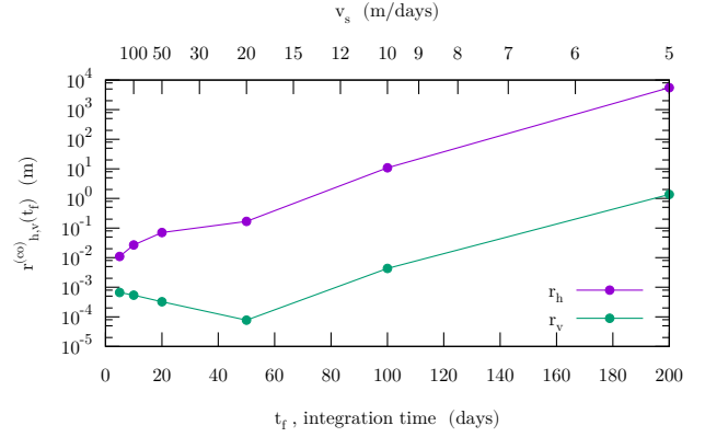
Figure 5. Root mean square difference per particle between final positions (at times t_f stated in Table 2) computed with and without the Coriolis term (Eqs. (10) and (9), respectively). Data are presented as a function of the unperturbed sinking velocity v_s used (upper horizontal scale) and of the final integration time t_f (lower horizontal scale). Upper violet line, the horizontal difference r_h^{(co)}(t_f) ; lower green line, the vertical difference r_v^{(co)}(t_f) .
