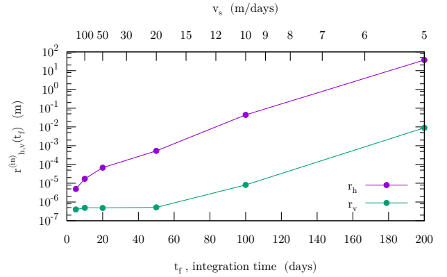
Figure 6. Root mean square difference per particle between final positions (at times t_f stated in Table 2) computed with and without the inertial term (Eqs. (11) and (9), respectively). Data are presented as a function of the unperturbed sinking velocity v_s used (upper horizontal scale) and of the final integration time t_f (lower horizontal scale). Upper violet line, the horizontal difference r_h^{(in)}(t_f) ; lower green line, the vertical difference r_v^{(in)}(t_f) .
