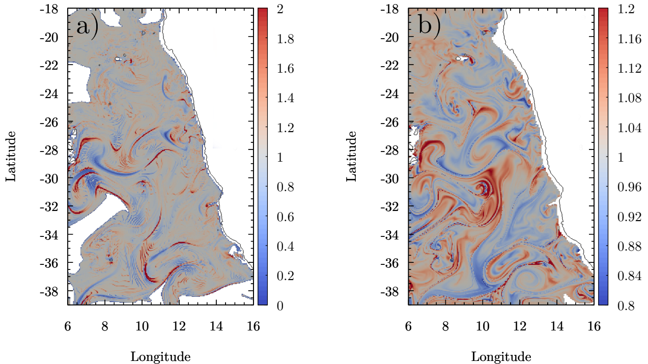
Figure 7. Results of the clustering numerical experiments of Sect. 5. a) N_f/N_0 , the number of particles N_f arriving to an horizontal box of size 1/25^\circ in the horizontal layer at z = -1000 m, normalized by the number of particles N_0 = 1000 released from the upper z = -100 m layer. b) The corrected dilation factor \delta(\mathbf{x}, t_f)^{-1} \cos(\theta_f)/\cos(\theta_0) mapped on the final z = -1000 m layer. It gives the ratio between horizontal densities at the final and initial locations, corrected with the latitudinal dependence of the horizontal boxes used in panel a), to give an estimation of the local particle number ratio between lower and upper layer. Black thin line represents the coastline; white oceanic areas indicate in a) regions which do not receive any falling particles; in b) regions from which the backward integration ends up outside the domain.
