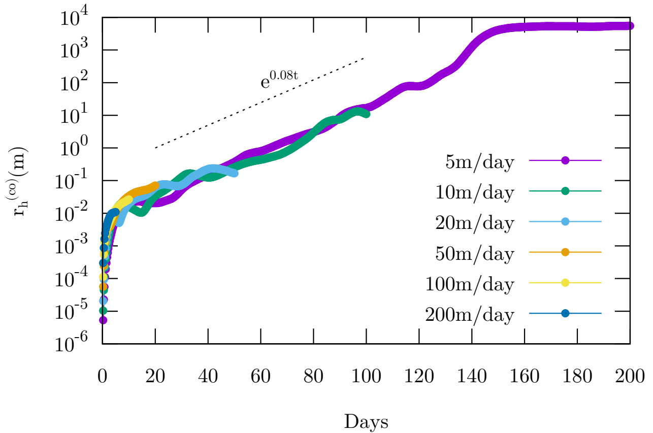
Figure 4. Root mean square difference per particle, as a function of time, between horizontal particle positions computed with Eq. (9) and with Eq. (10), i.e. with and without the Coriolis term. The different colors correspond to distinct values of the unperturbed sinking velocity. The dashed line is an exponential with slope 0.08 \text{ day}^{-1} .
