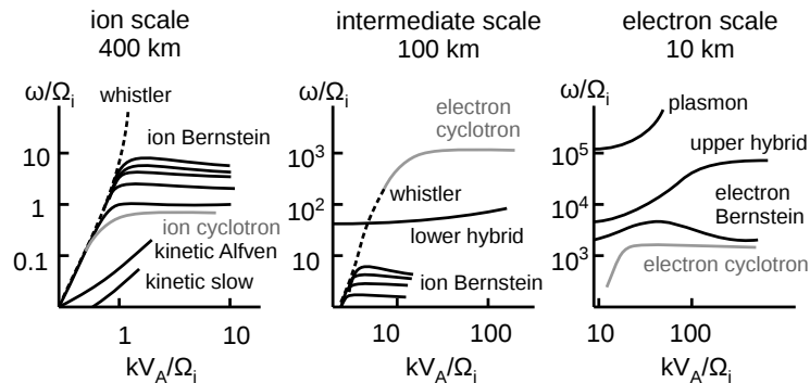
Figure 1. Schematic dispersion relations on ion-kinetic to electron-kinetic scales for oblique wave propagation to the mean magnetic field. Ion and electron cyclotron branches (in gray) are associated with the propagate direction parallel or oblique to the mean magnetic field. The other branches (in black) are for oblique to quasi-perpendicular directions to the mean field. Whistler branch can exist for the quasi-parallel, oblique, and quasi-perpendicular directions.
