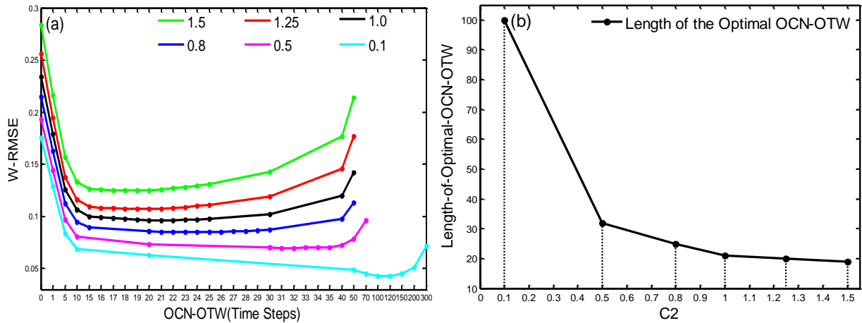
Figure 10: Panel (a) is same as panel (b) in Fig. 9 but for using six different coupling strength cases (with C_2 values as 1.5, 1.25, 1.0, 0.8, 0.5, 0.1 while C_1 keeps as 0.1). Panel (b) is the variation of the length of the optimal OCN-OTW with respect to the values of C_2 .
