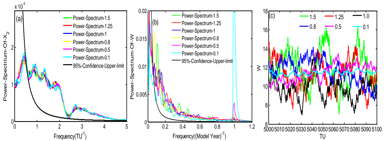
Figure 9: The power spectrum of (a) X_2 and (b) \omega based on the model states between 5000 TUs and 9800 TUs integrations after the spin-up which integrates for 10000TUs from the initial condition (0,1,0,0) with different coupling strength ( C_2 is set as 1.5, 1.25, 1.0, 0.8, 0.5 and 0.1 while C_1 keeps as 0.1). Panel (c) shows the time series of the model state \omega between 5000TUs and 5100TUs integrations corresponding to the six cases.
