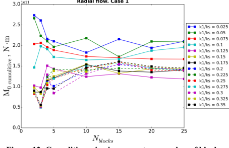
Figure 12: Cumulative seismic moment vs. number of blocks.
