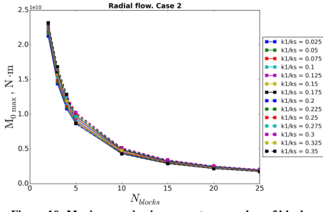
Figure 10: Maximum seismic moment vs. number of blocks.
