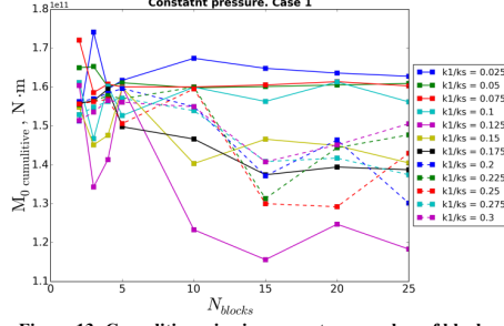
Figure 13: Cumulative seismic moment vs. number of blocks.
