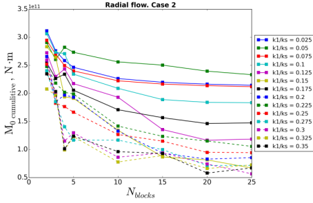
Figure 14: Cumulative seismic moment vs. number of blocks.
