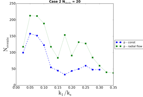
Figure 17: Event cumulative numbers dependence on the stiffnesses of the interblock link.
