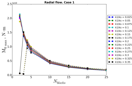
Figure 8: Maximum seismic moment of event vs. number of blocks.
