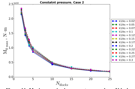
Figure 11: Maximum seismic moment vs. number of blocks.
