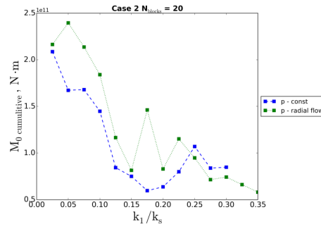
Figure 23: The block system cumulative seismic moment dependence on the stiffness of the interblock link.
