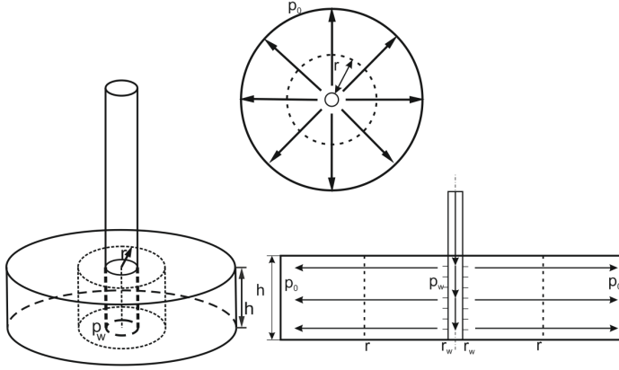
Figure 2: Radial flow in homogeneous reservoir.
