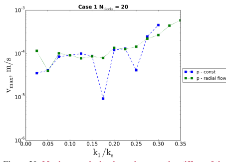
Figure 20: Maximum velocity dependence on the stiffnesses of the interblock link.
