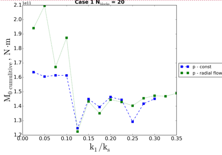
Figure 22: The block system cumulative seismic moment dependence on the stiffnesses of the interblock link.
