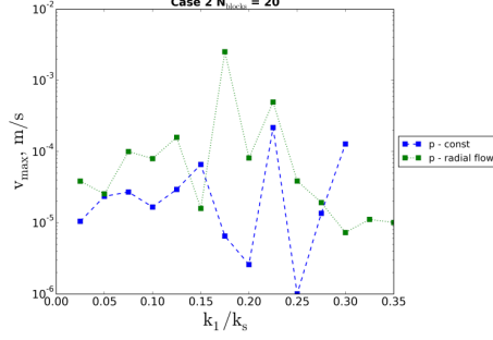
Figure 21: Maximum velocity dependence on the stiffnesses of the interblock link.
