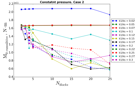
Figure 15: Cumulative seismic moment vs. number of blocks.
