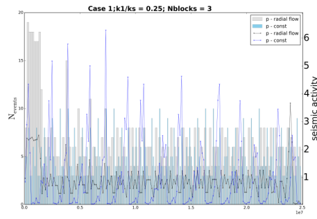
Figure 30: Time variation of seismic activity.
