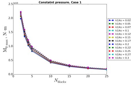
Figure 9: Maximum seismic moment of event vs. number of blocks.
