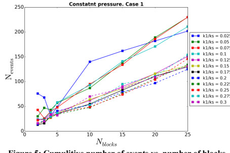
Figure 5: Cumulative number of events vs. number of blocks.
