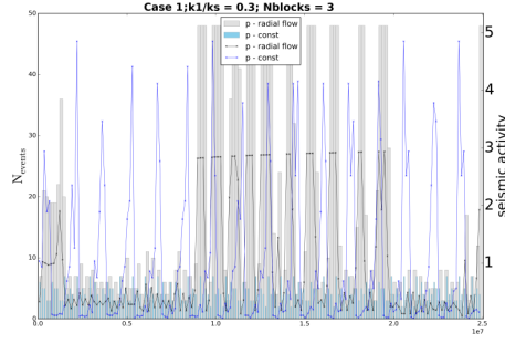
Figure 32: Time variation of seismic activity.
