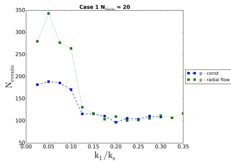
Figure 16: Event cumulative numbers dependence on the stiffnesses of the interblock link.
