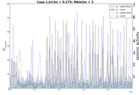
Figure 31: Time variation of seismic activity.
