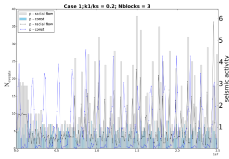
Figure 29: Time variation of seismic activity.
