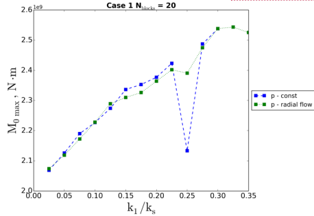
Figure 18: The event maximum seismic moment dependence on the stiffnesses of the interblock link.
