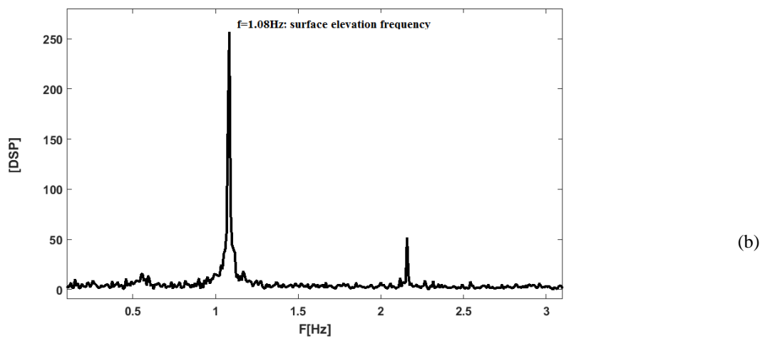
Figure 3. Power spectrum frequency: (a) in absence of breaking waves: the first peak indicates the edge wave frequency, while the second peak indicates the surface elevation frequency; (b) in presence of breaking waves: the peak for the edge wave frequency is suppressed.
