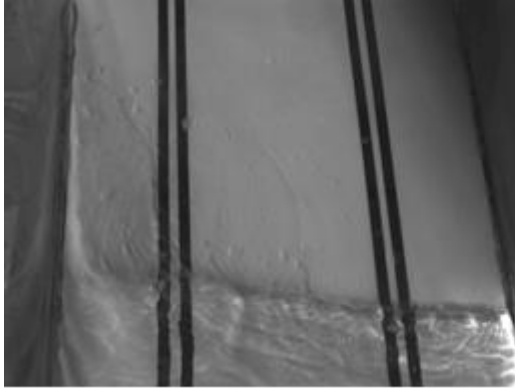
15 Figure4. Snapshots of water surface over the time interval equal to a half of the edge wave period (approximately 1 s), f = 1.06 Hz, a_L = 1.3 cm.
