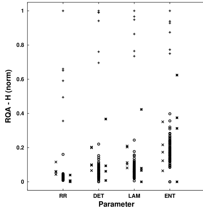
Figure 7. Normalized representation of the RQA parameters for Auroral Electrojet AE indices in HILDCAA events (o), in CIR/HSS not followed by HILDCAA (x), in a global geomagnetic disturbance scenario (*), and in the geomagnetically quieter intervals (+).
