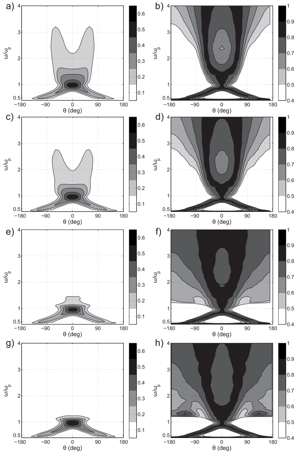
Figure 7. Isolines of spreading functions for different runs (see Table 1) a,b ) – sw030 ; c,d ) – sw170 ; e,f ) – sw330 ; g,h ) – run sw330 with finer resolution in angle \Delta\theta = 5^\circ . Left column – definition (32), right – (33).
