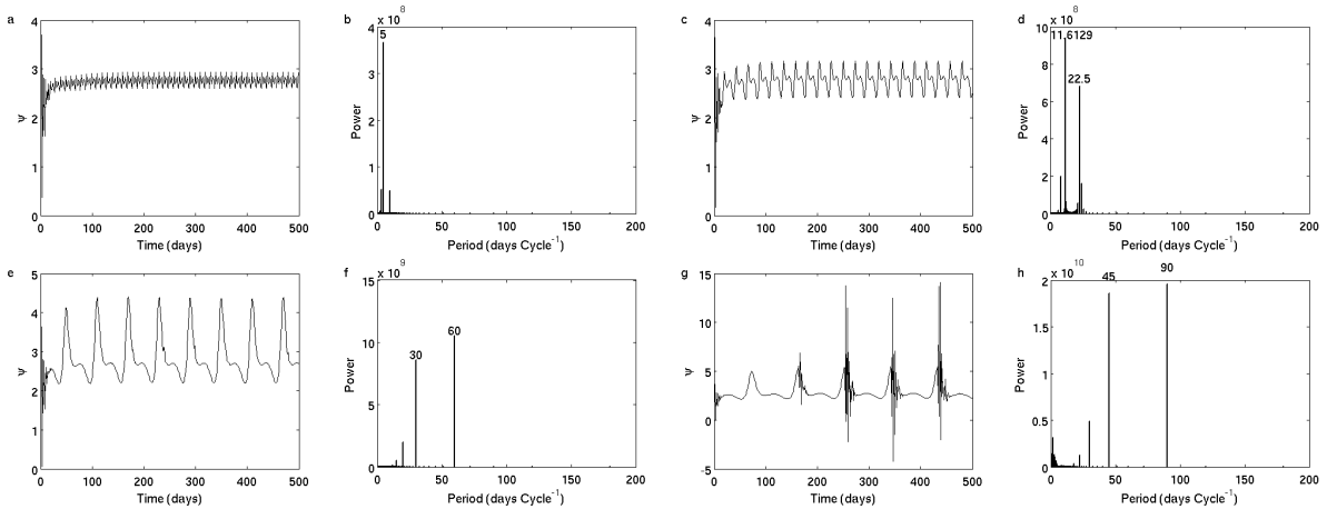
Figure 1. Temporal evolution of the stream-function at 3^\circ North and 2400 m (a,c,e) and its power spectral density (b,d,f) when t_0 = 10 (a,b), 23 (c,d) 60 days (e,f) and 90 days(g,h). The figures on the bars are the cycle periods in days.
