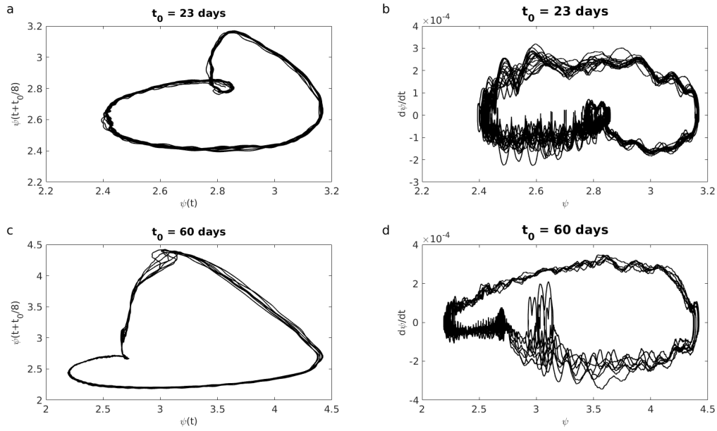
Figure 2. Representation of the evolution of the stream-function at 3^\circ North and 2400 m \psi(t)-\psi(t+t_0/8) (left panels) for t_0 = 23 days (upper panels) and t_0 = 60 days experiments (lower panels).
