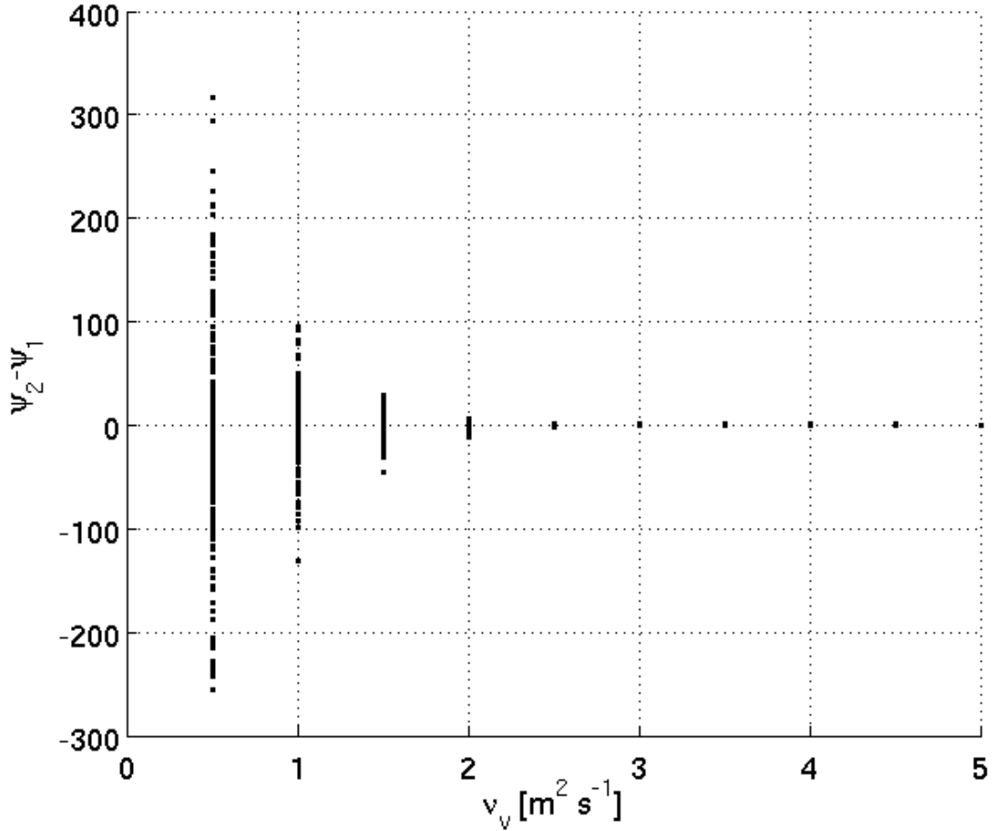
Figure 11. The 1-D bifurcation diagram as a function of \nu_v for simulations with t_0 = 30 days.
