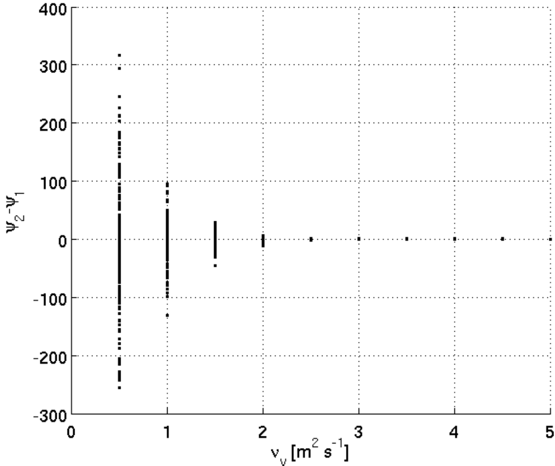
Figure 11. The 1-D bifurcation diagram as a function of \nu_v for simulations with t_0 = 30 days.
