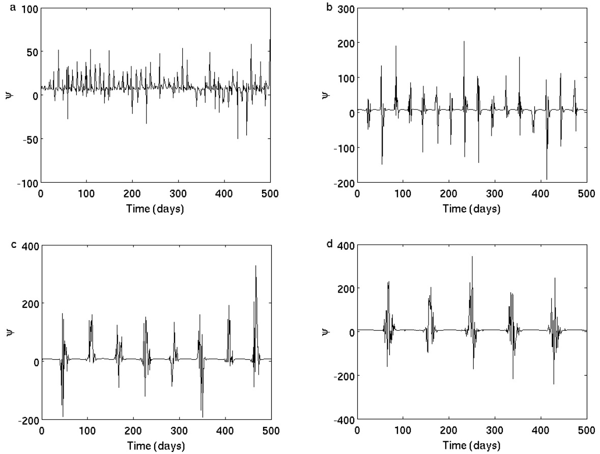
Figure 9. The time evolution of stream-function (in dimensionless unit) at 3^\circ North and 2400 m for t_0 = 10 (a), 30 (b), 60 (c) and 90 (d) when \nu_V = 0.5 .
