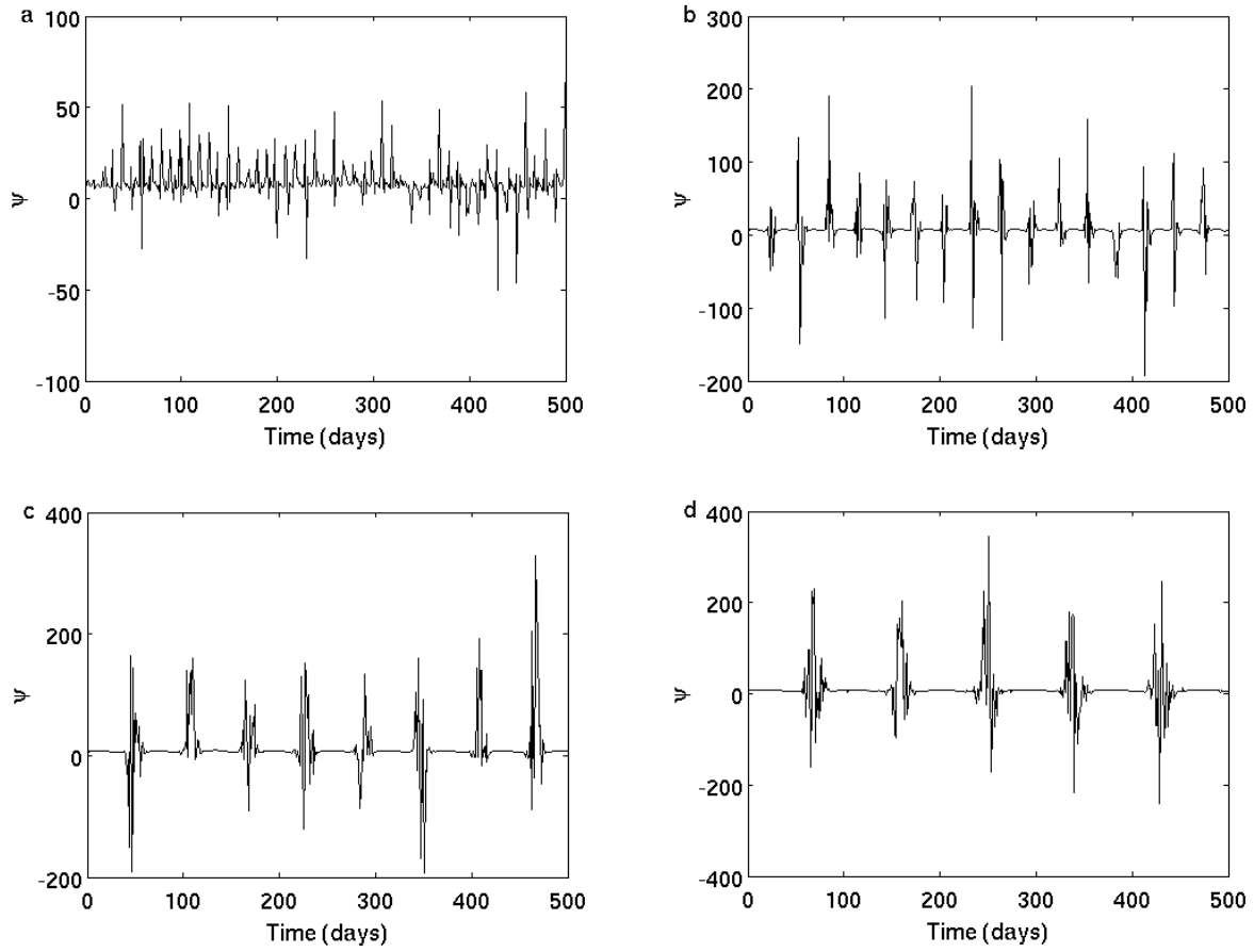
Figure 10. The time evolution of stream-function (in dimensionless unit) at 3° North and 2400 m for t_0 = 10 (a), 30 (b), 60 (c) and 90 (d) when \nu_V = 0.5 .
