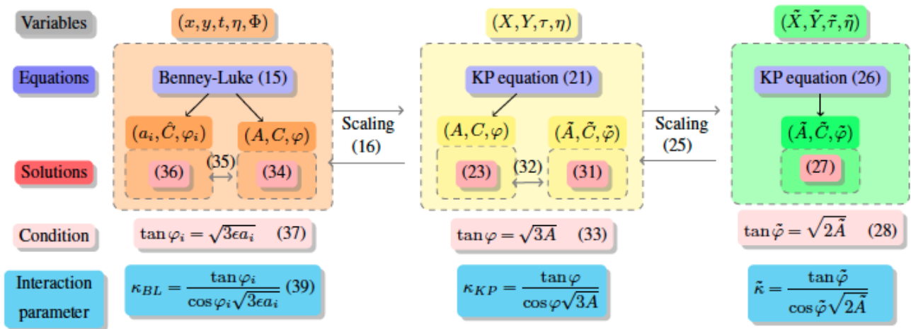
Figure 4. Schematic plan showing the link between the scaling of the three system of equations involved in the derivation of the exact solution and critical condition for which Miles' and Kodama's predictions hold in the Benney-Luke approximation.
