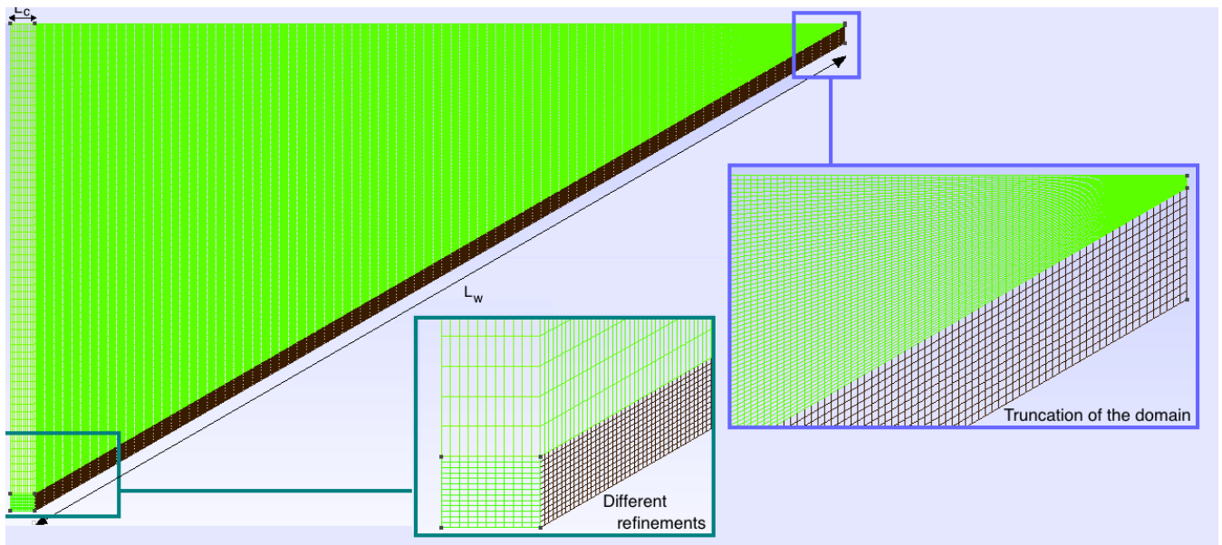
Figure 7. Domain discretisation using quadrilaterals in Gmsh. In order to reduce computational requirements, mesh refinement is restricted to only the region adjacent to the wall.
