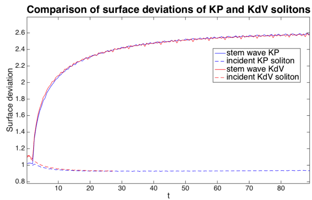
Figure 6. Soliton surface deviations obtained for an initial amplitude a_i = 1.0 , and angle \varphi_i = \pi/6 rad. Blue: behaviour of the incident (dashed line) and stem (full line) waves when the incident soliton propagates in an oblique direction; red: behaviour of the incident (dashed line) and stem (full line) waves when the incident soliton propagates in one direction. The dashes lines essentially coincide after t > 30 .
