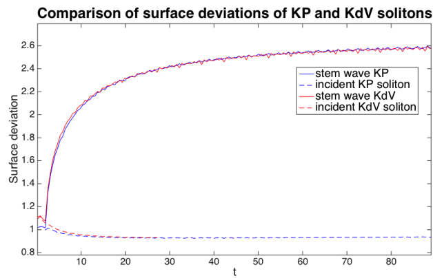
Figure 6. Soliton surface deviations obtained for an initial amplitude a_i = 1.0 , and angle \varphi_i = \pi/6 rad. Blue: behaviour of the incident and stem waves when the incident soliton propagates in an oblique direction; red: behaviour of the incident and stem waves when the incident soliton propagates in one direction.
