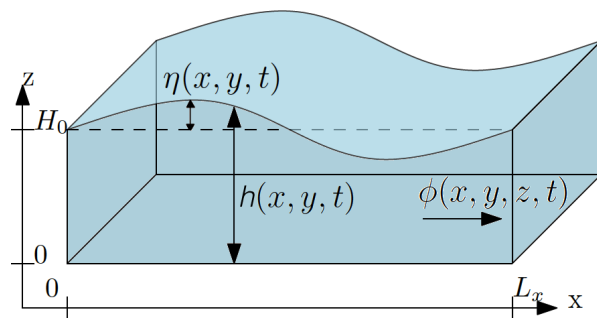
Figure 2. Three-dimensional water-wave domain with rest-depth H_0 . We aim to estimate the potential \phi(x, y, z, t) and the free-surface deviation \eta(x, y, t) from the rest depth.
