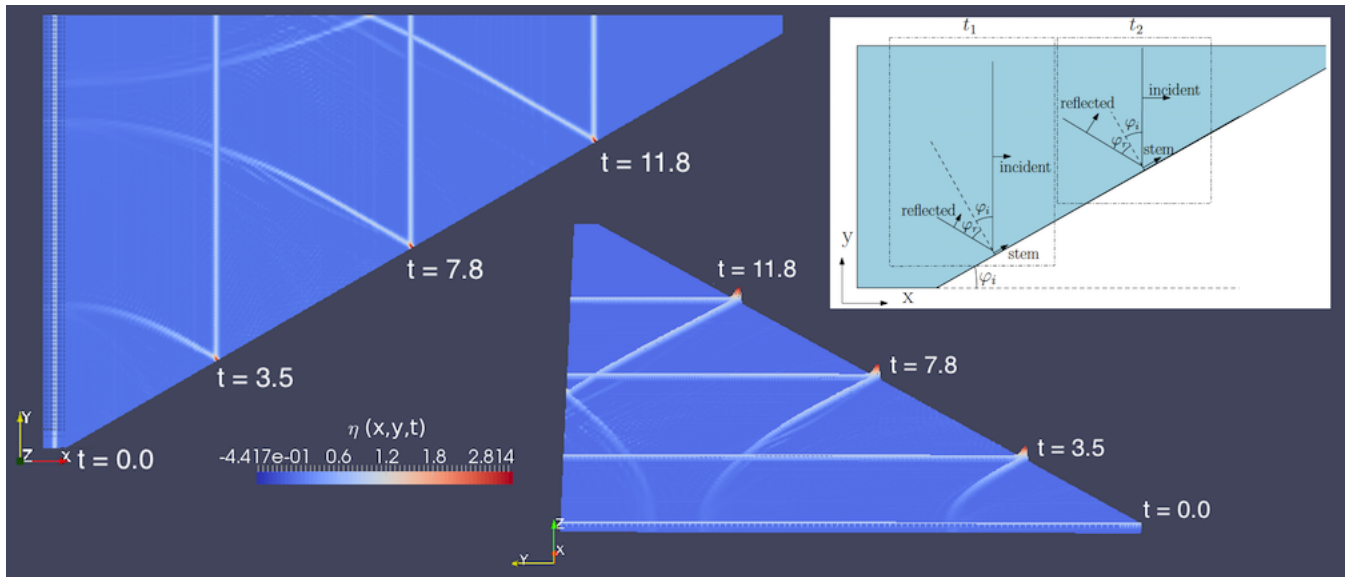
Figure 9. Numerical results and expectations for the reflected and stem waves in the case of regular reflection, that is \kappa > 1 . Left: top view of the numerical evolution of the incident, reflected and stem waves. Top right: top view of the expected evolution of the stem and reflected waves at two different times t_1 and t_2 with t_1 < t_2 . The stem wave should propagate along the wall with constant length. The angle \varphi_r of the reflected wave is expected to be constant and equal to the incident wave's angle \varphi_i . Bottom right: side view of the time evolution of the incident, reflected and stem waves highlighting the amplification of the stem wave's amplitude compared to the initial solitary wave's height.
