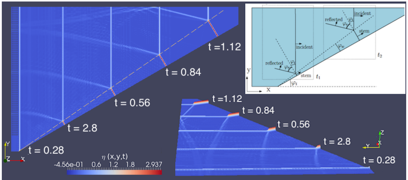
Figure 10. Numerical results and expectations for the reflected and stem waves in the case of Mach reflection, that is \kappa < 1 . Left: top view of the numerical evolution of the incident, reflected and stem waves. Top right: top view scheme of the expected evolution of the stem and reflected waves at two different times t_1 and t_2 with t_1 < t_2 . The stem wave should linearly grow in length, leading to an angle \varphi_w > 0 rad with the wall. The angle \varphi_r of the reflected wave is expected to be constant and larger than the incident wave's angle \varphi_i . Bottom right: side view of the time evolution of the incident, reflected and stem waves highlighting the amplification of the stem wave's amplitude compared to the initial solitary wave's height.
