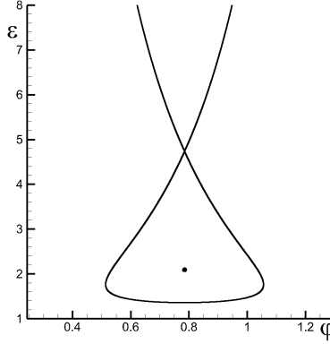
Figure 1. The phase portrait of the stationary system (1) in the case of one elliptic and one hyperbolic critical points for e_0 = 0.15 , \gamma_0 = 0.02 .
