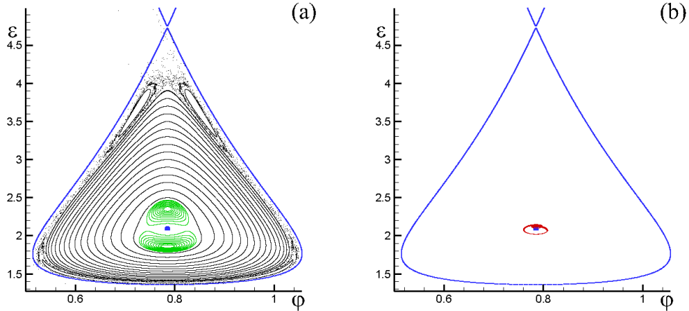
Figure 3. The dynamics of the perturbed system in the case of the primary parametric instability zone of the corresponding linearized system (7) for e_0 = 0.15 , \gamma_0 = 0.02 and perturbation parameters \delta = 0.01 , \nu = 0.6 . The solid blue lines show the steady-state separatrix. The blue dot shows the steady-state elliptic critical point \varphi_0 = \pi/4 , \varepsilon_0 \approx 2.09244 . (a) a Poincaré section illustrating the appearance of a highly nonlinear zone (the green orbits) near the steady-state elliptic critical point that prohibits the divergent motion due to the linear parametric resonance; (b) a phase trajectory starting at the steady-state elliptic critical point bounded to the region of the nonlinear resonance illustrating a vanishing effect of the linear parametric resonance.
