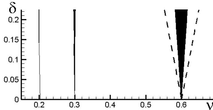
Figure 2. The regions of parametric instability in the parametric plane \nu, \delta for e_0 = 0.15, \gamma_0 = 0.02 . The dark regions correspond to locally unbounded dynamics of the ellipse obtained with the use of the linear approximation (7). The dashed lines mark the region incurred from the analytical estimate (12).
