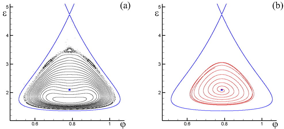
Figure 4. The same as in fig. 3 except \nu = 0.3 . (a) a Poincaré section illustrating that the perturbed system remains largely linear near the steady-state elliptic critical point; (b) a divergent spiralling phase trajectory starting at the steady-state elliptic critical experiencing linear parametric instability.
