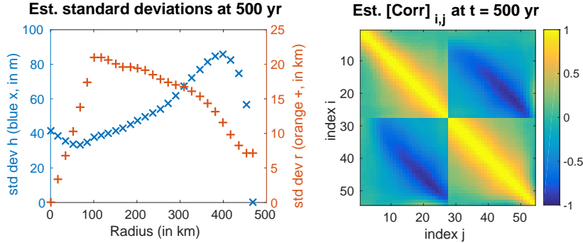
Figure 8. Standard deviations and correlation matrix Corr estimated from the ETKF analysis ensemble at time t = 500 yr when we use only observations of ice thickness. Auto-correlations between ice thicknesses are located in the top left corner of Corr , auto-correlations between node positions in the bottom right corner. The rest of the matrix depicts the cross-correlations.
