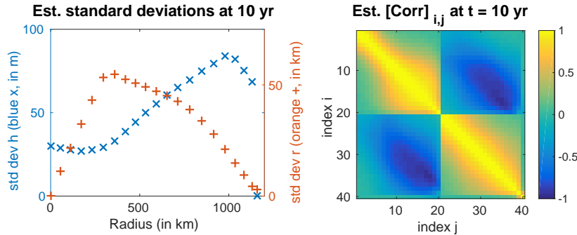
Figure 14. Standard deviations and correlation matrix Corr estimated from the analysis ensemble at time t = 10 yr in the advanced configuration where we observe surface elevation. The matrix Corr has the same structure as B defined by Eq. (28). Both standard deviations and correlation structures are similar to Fig. 8.
