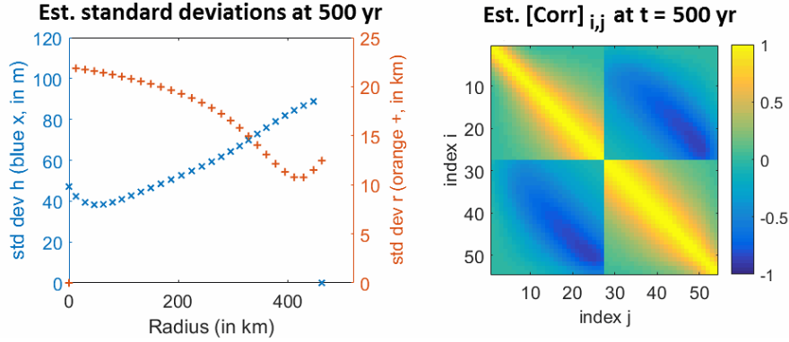
Figure 6. Standard deviations and correlation matrix Corr estimated from the 3DVar analysis at time t = 500 yr when we use only observations of ice thickness. Auto-correlations between ice thicknesses are located in the top left corner of Corr , auto-correlations between node positions in the bottom right corner. The rest of the matrix depicts the cross-correlations.
