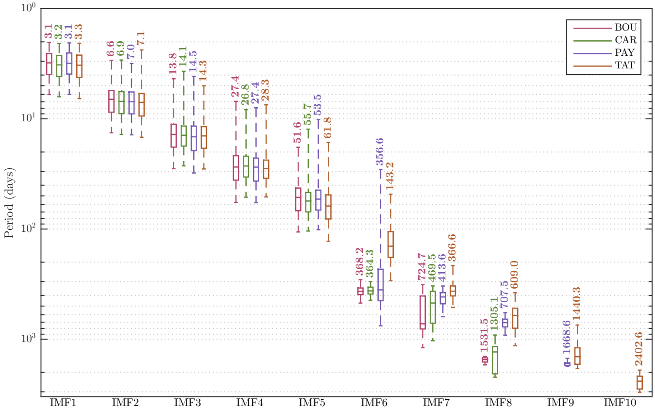
Figure 7. Box plot of the instantaneous time-scales of the IMFs for the four stations. The top and the bottom edges of the boxes represent the first ( Q1 ) and, respectively, the third ( Q3 ) quartiles. The bars inside boxes denote the second quartile ( Q2 ), i.e. the median. The whisker length is set at at most 1.5 times the interquartile range, i.e. 1.5 \times (Q3 - Q1) , hence the whiskers roughly correspond to \pm 2.7 standard deviations, or equivalently \sim 99\% of the data, assuming normal distribution. The median for each box is expressed numerically above the lower whiskers. Outliers are omitted. Numeric values for all the statistical descriptors are shown in table 2.
