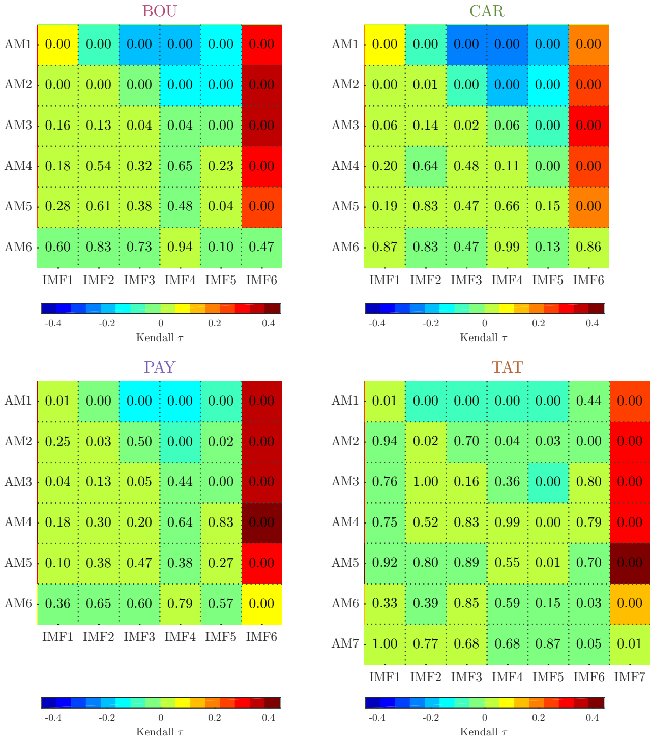
Figure 10. Rank correlations between IMFs and their AM components for BOU (top left), CAR (top right), PAY (bottom left) and TAT (bottom right). Kendall’s rank correlation coefficient \tau is colour-coded according to the colour bar on the bottom. IMFs run vertically, along the columns, and their AM components run horizontally, along the rows. The numeric values within the cells are the associated p -values.
