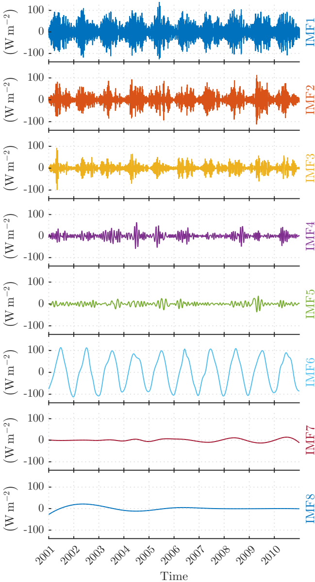
Figure 3. The eight IMFs obtained by decomposing the BOU time-series, from top to bottom IMF1...IMF8. The panels plot SSI (ordinate) versus time (abscissa). Time markers on the horizontal axes indicate January 1 st of the corresponding year. The zero-centred oscillatory nature of the modes can be clearly seen. Also apparent is the local time-scale increase with mode number.
