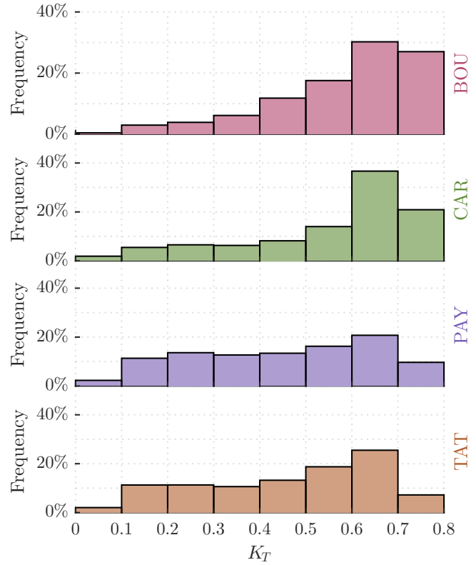
Figure 2. Histograms of the daily clearness index K_T over the decennial time-span in frequency in percent. From top to bottom: BOU, CAR, PAY, and TAT.
