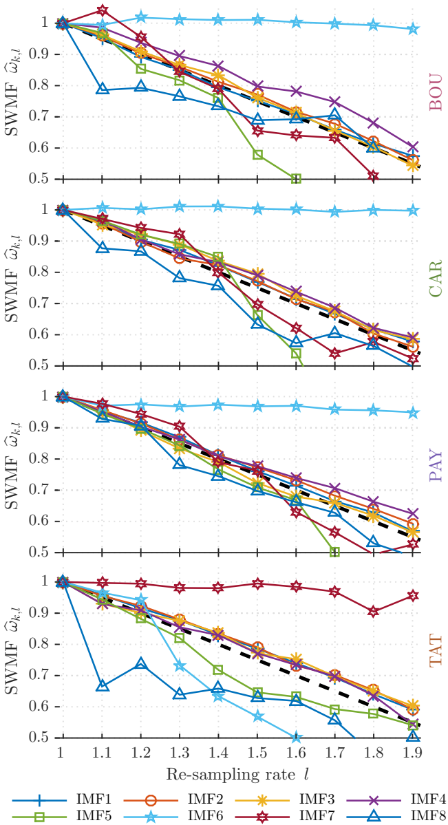
Figure 9. The drift of normalized SWMF \hat{\omega}_{k,l} (ordinate) of IMF k , with k \in \{1 \dots 8\} , as a function of the re-sampling rate l (abscissa) for the four time-series. From top to bottom: BOU, CAR, PAY, and TAT. The black dashed diagonal depicts the behaviour of a pure noise time-series under an ideal dyadic filter. For all datasets, the only mode that maintains a quasi-constant frequency under fractional re-sampling is the IMF associated with the yearly cycle, i.e. IMF6 for BOU, CAR, and PAY and IMF7 for TAT. In all the other IMFs quasi-stochastic behaviour is apparent, through frequency down-shifting towards the next lower octave, approximately following the dashed line.
