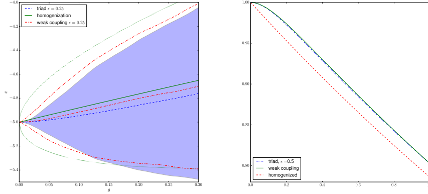
Figure 2. Left: comparison of the ensemble spread for the original additive triad system for \varepsilon = 0.25 from an initial condition (-5, 0, 0) (the ensemble mean is the blue dashed line, 2\sigma interval the blue shaded area), the two-level Ornstein-Uhlenbeck process from the weak coupling method (11) from an initial condition (-5, 0) (ensemble mean: red dash-dotted line, 2\sigma interval: red dash-dot-dotted lines) and the one-level Ornstein-Uhlenbeck process from homogenization (4) from x = -5 (ensemble mean: green solid line, 2\sigma interval: dotted lines) Right: comparison of the autocorrelation functions of the slow variable \langle x(t)x(0) \rangle in the full triad for \varepsilon = 0.5 (blue dash-dotted line), \langle z_1(t)z_1(0) \rangle in the weak coupling model (green solid line) and \langle x(t)x(0) \rangle for the homogenized equation (red dashed line). Both plots use parameter values B^{(0)} = -0.75 , B^{(1)} = -0.25 , B^{(2)} = 1 , \gamma_1 = 1/\delta , \sigma_1 = \sqrt{2/\delta} , \gamma_2 = 1 and \sigma_2 = \sqrt{2} with \delta = 0.75 .
