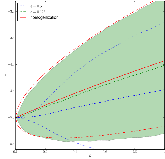
Figure 1. Convergence to the homogenized equations for the additive triad (3) in \theta = \varepsilon t time scale. The red solid and dash-double-dotted lines show the mean and 2\sigma intervals respectively for an ensemble evolving according to the homogenized equation (4) from an initial condition x = -5 . The blue dashed and dotted lines show the mean and 2\sigma intervals for an ensemble of the additive triad (3) for \varepsilon = 0.5 from an initial condition (x, y_1, y_2) = (-5, 0, 0) with B^{(0)} = -0.75 , B^{(1)} = -0.25 , B^{(2)} = 1 , \gamma_1 = 1/\delta , \sigma_1 = \sqrt{2/\delta} , \gamma_2 = 1 and \sigma_2 = \sqrt{2} with \delta = 0.75 . The green dash-dotted line and the green shaded area show the same for \varepsilon = 0.125 .
