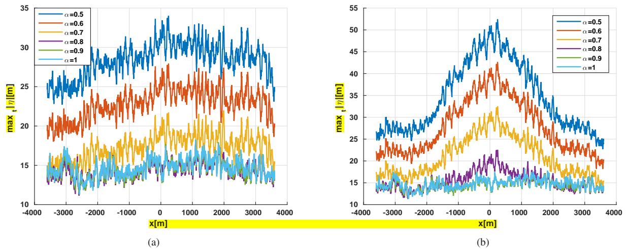
Figure 3. The maximal temporal amplitude of the linear evolution of the wpm signal for various values of \alpha . Figure (a) corresponds to restricting the phases to a quart stdv, |\omega - \omega_p| < 0.25\sigma_\omega and (b) for a half stdv, |\omega - \omega_p| < 0.5\sigma_\omega .
