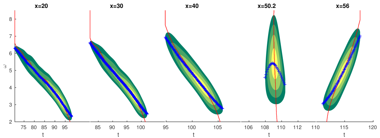
Figure 8. Case 202002. A filled contour plot of the energy distribution of the critical group event at position x = 20, 30, 40, 50.2, 56 . At each position the red solid lines show the time of maximal energy at each wave frequency. The '+' lines show the wave frequency as function of time. Both are estimated by the most energetic waves in time and in frequency respectively. Before x = 50.2 both solid and '+' lines show decreasing frequencies (increasing wave length) in time, then it leads to energy convergence.
