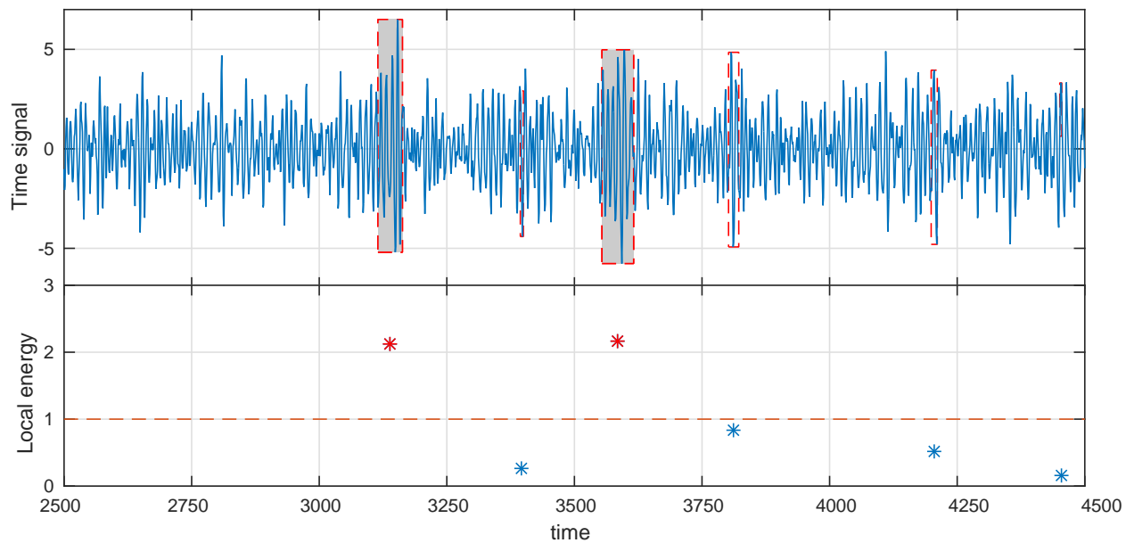
Figure 10. Case W100. Initial time signal in the interval t \in [2500, 4500] . The critical group events are shown in the shaded areas of the upper plot. The lower plot presents the amount of local energy signal of the recognized group events compared to the local energy threshold (dashed line). The local energy signal of the critical group events are above the threshold.
