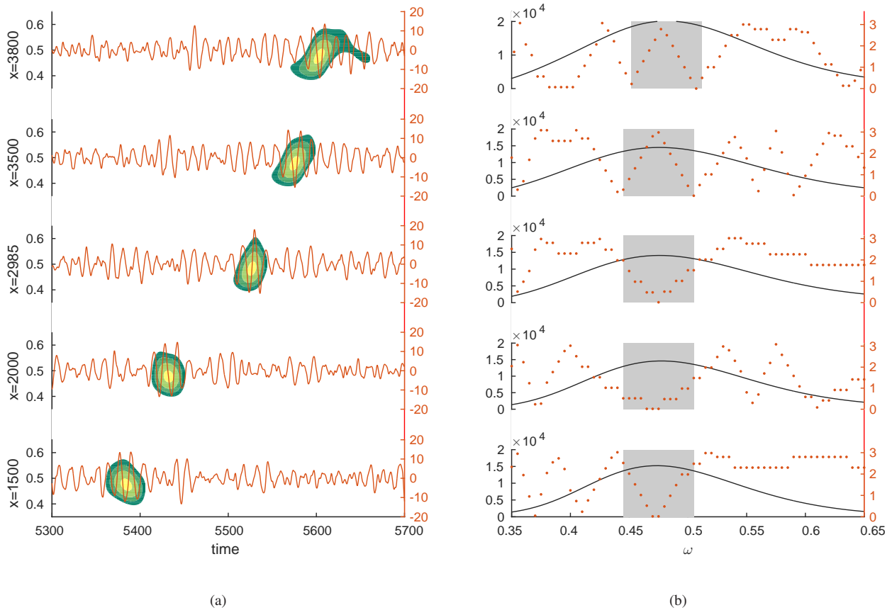
Figure 15. Case TS10000. (a) Time signals at various positions of the evolution of the critical group event with the filled contour plot of wavelet spectra. (b) The corresponding time-averaged wavelet spectra (solid line) and the time spreading (dotted line). The shaded areas show the chosen frequency interval of the most energy carrying modes.
