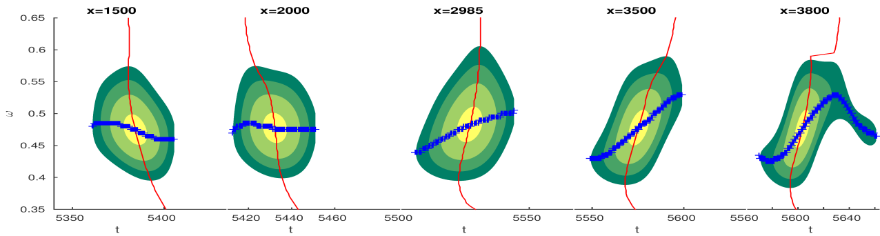
Figure 17. Case TS10000. A filled contour plot of the energy distribution of the critical group event at various positions. At each position the red solid lines show the time of maximal energy at each wave frequency. The '+' lines show the wave frequency as function of time. Both are estimated by the most energetic waves in time and in frequency respectively.
