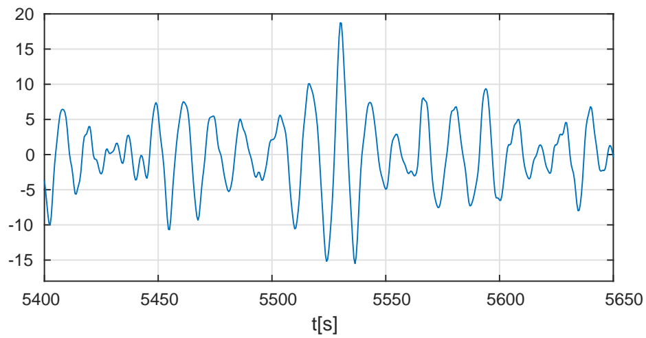
Figure 16. Case TS10000. Zoomed version of the freak wave; the crest height is 1.22 and the wave height is 2.23 times the significant wave height.
