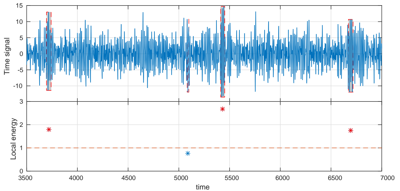
Figure 14. Case TS10000. Initial time signal in the interval t \in [3500, 7000] . The critical group events are shown in the shaded areas of the upper plot. The lower plot presents the amount of local energy signal of the recognized group events compared to the local energy threshold (dashed line). The local energy signal of the critical group events are above the threshold.
