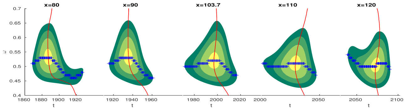
Figure 21. Case IW12. A filled contour plot of the energy distribution of the group event at various positions. At each position the red solid lines show the time of maximal energy at each wave frequency. The '+' lines show the wave frequency as function of time. Both are estimated by the most energetic waves in time and in frequency respectively.
