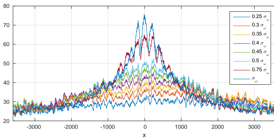
Figure 4. The maximal temporal amplitude of the linear evolution of the wpm signal with \alpha = 0.5 for various fractions of the standard deviation \sigma_\omega .
