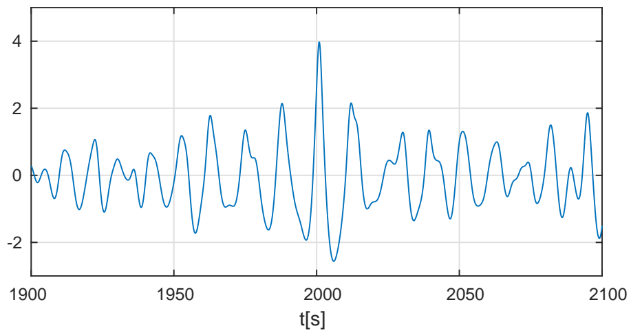
Figure 20. Case IW12. Zoomed version of the freak wave; the crest height is 1.31 and the wave height is 2.15 times the significant wave height.
