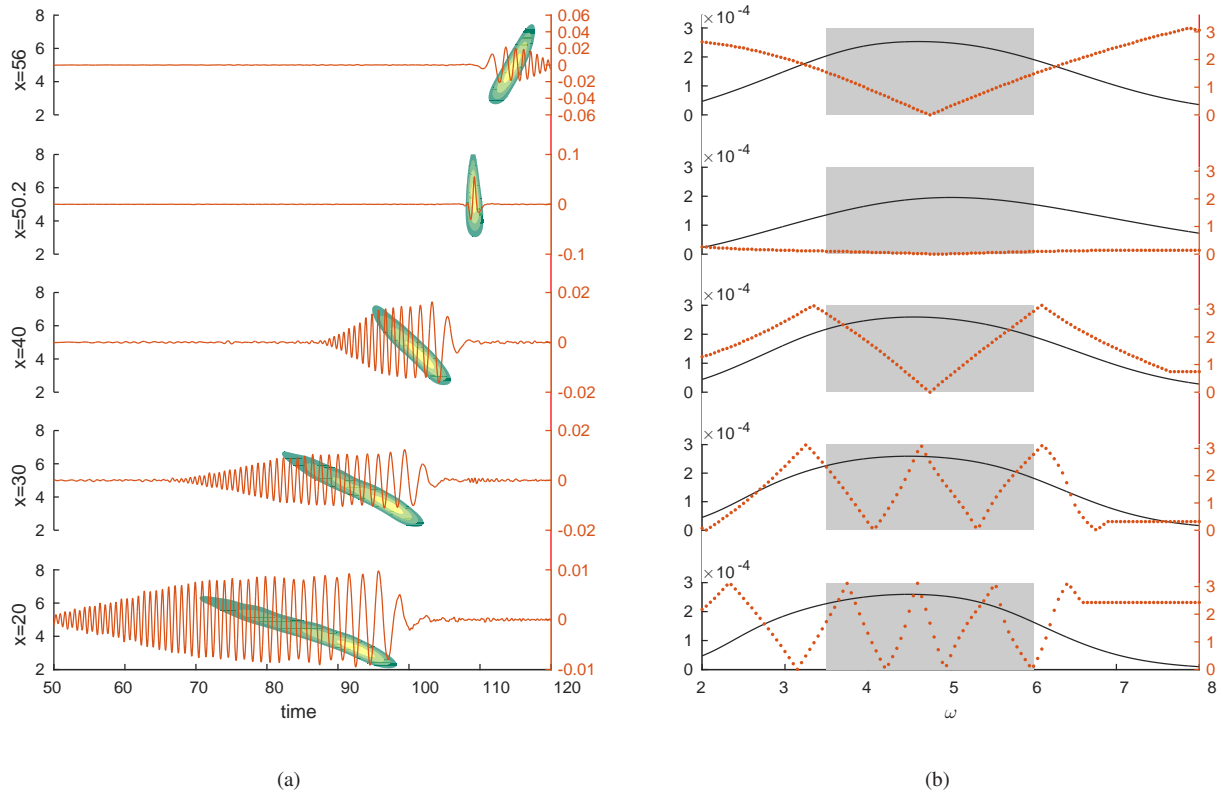
Figure 7. Case 202002. (a) Time signals at various positions of the evolution of the critical group event with the filled contour plot of wavelet spectra. The vertical axis at the left represents the wave frequency \omega and the vertical axis at the right represents the surface elevation in meters. (b) The corresponding time-averaged wavelet spectra (solid line) and the time spreading (dotted line). Observe that at x = 50.2 the time spreading vanishes identically in the shaded area. The shaded areas show the chosen frequency interval of the most energy carrying modes.
