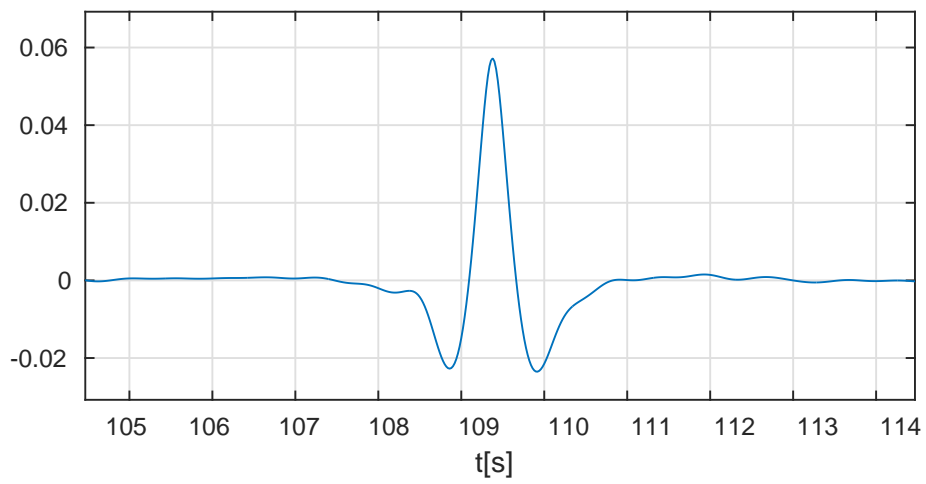
Figure 9. Case 202002. Zoomed version of the maximal wave; the crest height is 4.65 and the wave height is 6.56 times the significant wave height.
