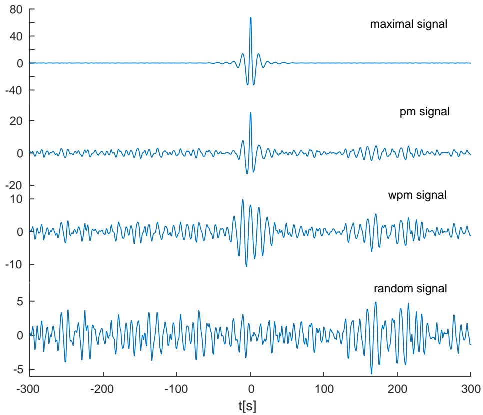
Figure 2. Shown are plots from up to down of a maximal, pseudo-maximal, and weak-pseudo maximal signal corresponding to the same random signal at the bottom. The random signal corresponds to a Jonswap spectrum with H_s = 6.3\text{m} and \gamma = 1.9 . The pm and wpm signals correspond to the value \alpha = 0.7 .
