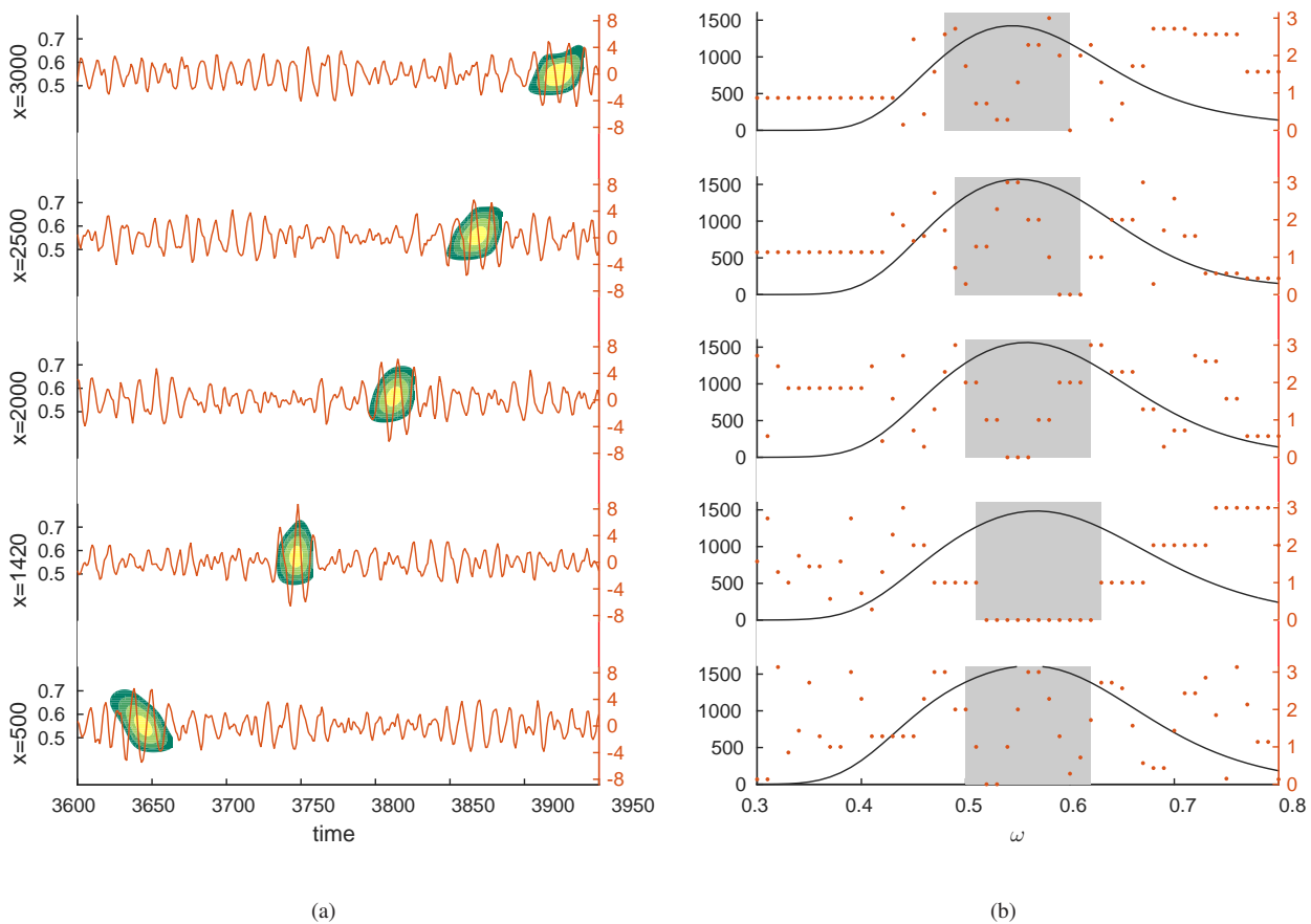
Figure 11. Case W100. (a) Time signals at various positions of the evolution of the critical group event with the filled contour plot of wavelet spectra. (b) The corresponding time-averaged wavelet spectra (solid line) and the time spreading (dotted line). Observe that at x = 1420\text{m} the time spreading is zero in the shaded area. The shaded areas show the chosen frequency interval of the most energy carrying modes.
