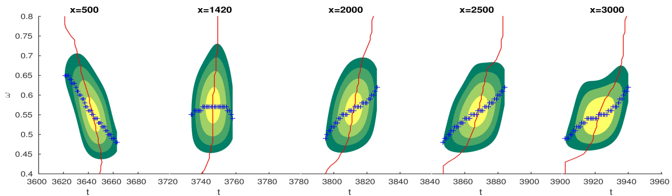
Figure 13. Case W100. A filled contour plot of the energy distribution of the critical group event at various positions. At each position the red solid lines show the time of maximal energy at each wave frequency. The '+' lines show the wave frequency as function of time. Both are estimated by the most energetic waves in time and in frequency respectively. Both lines show a decreasing frequency before the freak wave and an increasing frequency after the freak wave, while the freak wave occurs at x = 1420\text{m} .
