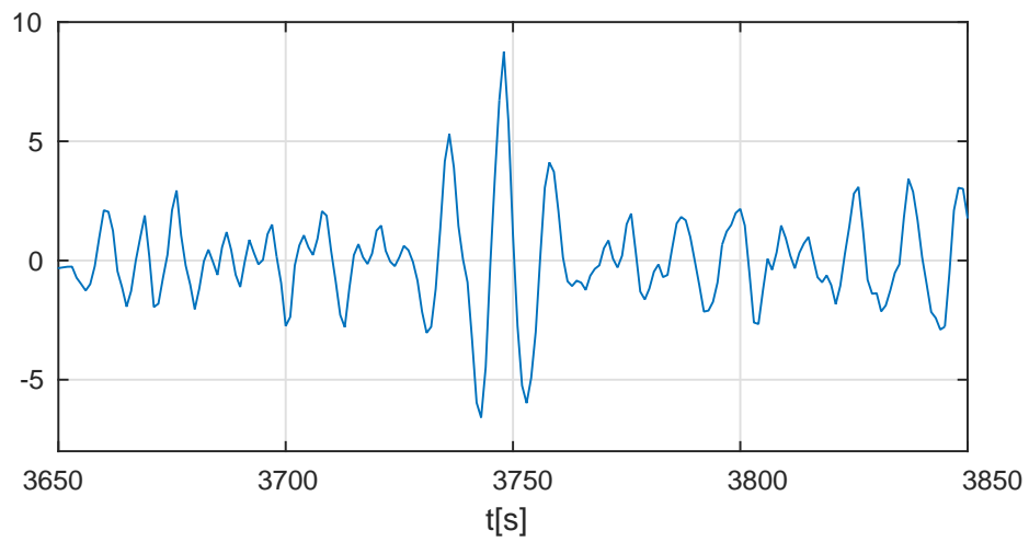
Figure 12. Case W100. Zoomed version of the freak wave; the crest height is 1.35 and the wave height is 2.37 times the significant wave height.
