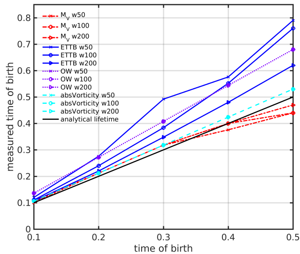
Figure 5. Time of birth of an eddy estimated with Okubo-Weiss (OW, violet), modulus of vorticity (absVorticity, cyan), M_V (red) and the eddy tracking tool box (ETTB, blue) by Nencioli et al. (2010) for vortex strength w 50, 100 and 200. The black diagonal depicts the analytical time of birth of an eddy.
