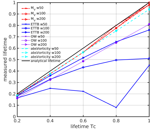
Figure 4. Eddy lifetime estimated with Okubo-Weiss (OW, violet), modulus of vorticity (absVorticity, cyan), M_V (red) and the eddy tracking tool box (ETTB, blue) by Nencioli et al. (2010) for vortex strength w 50, 100 and 200. The black diagonal depicts the analytical lifetime.
