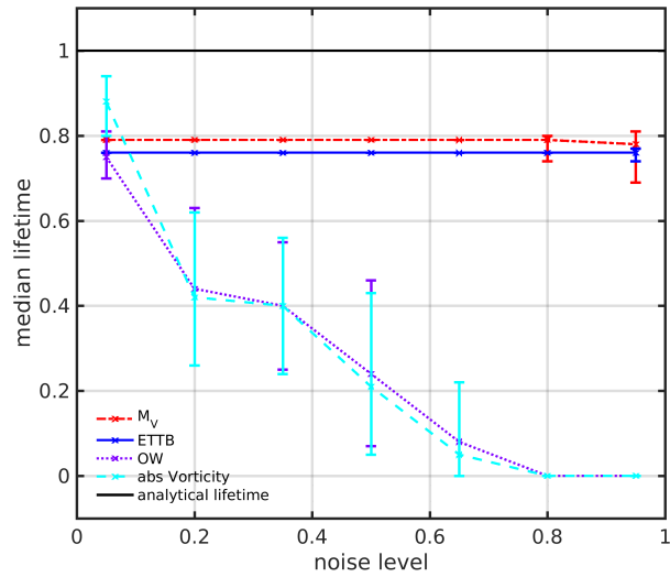
Figure 7. Measured median lifetime obtained by different methods (Okubo-Weiss (OW, violet), modulus of vorticity (absVorticity, cyan), M_V (red) and the eddy tracking tool box (ETT B, blue) by Nencioli et al. (2010)) depending on the noise level. The computations have been performed in a velocity field mimicking a vortex street with added white Gaussian noise (type 1 noise with 1000 noise realizations). The errorbars indicate the whiskers of the distribution in the boxplot (not shown here) corresponding to approximately \pm 2.7\sigma .
