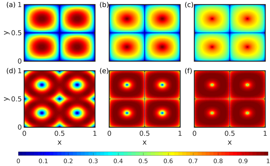
Figure 2. Colour-coded representation of the Lagrangian descriptor M_V (a)-(c) and the Lagrangian descriptor M (d)-(f) for the eddy field in Eq. (6) with \tau chosen as 0.5 ((a) and (d)), 25 ((b) and (e)) and 100 ((c) and (f)). All plots are normalized to the maximum value.
