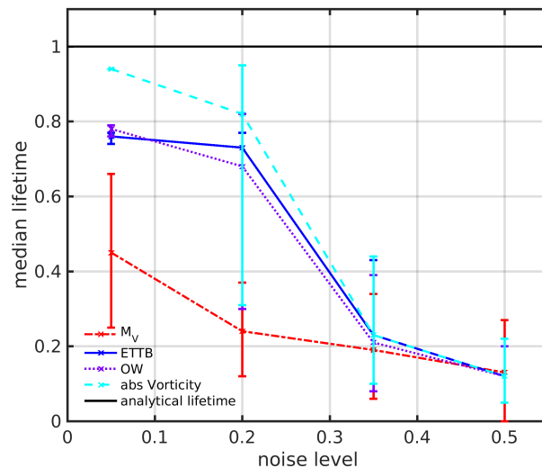
Figure 9. Measured median lifetime obtained by different methods (Okubo-Weiss (OW, violet), modulus of vorticity (absVorticity, cyan), M_V (red) and the eddy tracking tool box (ETTB, blue) by Nencioli et al. (2010)) depending on the noise level. The computations have been performed in a velocity field mimicking a vortex street with type 3 noise (1000 noise realizations). The errorbars indicate the whiskers of the distribution in the boxplot (not shown here) corresponding to approximately \pm 2.7\sigma .
