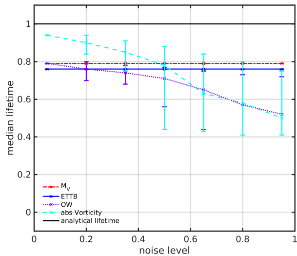
Figure 8. Measured median lifetime obtained by different methods (Okubo-Weiss (OW, violet), modulus of vorticity (absVorticity, cyan), M_V (red) and the eddy tracking tool box (ETTB, blue) by Nencioli et al. (2010)) depending on the noise level. The computations have been performed in a velocity field mimicking a vortex street with type 2 noise (1000 noise realizations). The errorbars indicate the whiskers of the distribution in the boxplot (not shown here) corresponding to approximately \pm 2.7\sigma .
