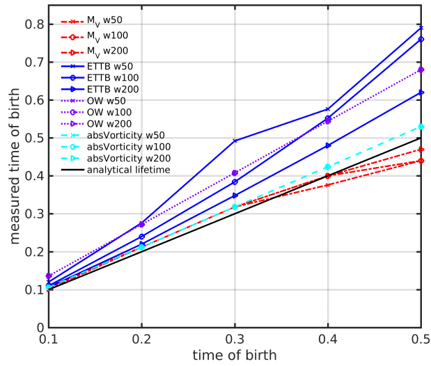
Figure 5. Time of birth of an eddy estimated with Okubo-Weiss (OW), modulus of vorticity (absVorticity), M_V and the eddy tracking tool box (ETT B ) by Nencioli et al. (2010) for vortex strength w 50, 100 and 200. The black diagonal depicts the analytical time of birth of an eddy.
