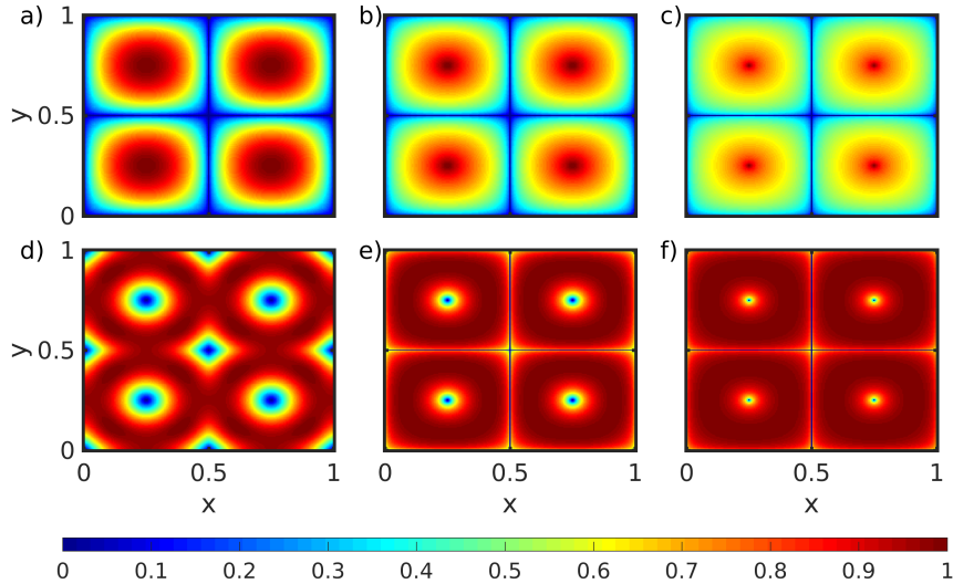
Figure 2. Colour-coded representation of the Lagrangian descriptor M_V (a-c) and the Lagrangian descriptor M (d-f) for the eddy field in Eq. (6) with \tau chosen as 0.5 (a and d), 25 (b and e) and 100 (c and f). All plots are normalized to the maximum value.
