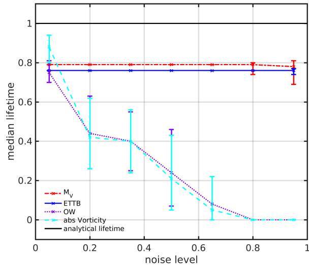
Figure 7. Measured median lifetime obtained by different methods (Okubo-Weiss (OW, violet), modulus of vorticity (absVorticity, cyan), M_V (red) and the eddy tracking tool box (ETTB, blue) by Nencioli et al. (2010)) depending on the noise level. The computations have been performed in a velocity field mimicking a vortex street with added white Gaussian noise (type 1 noise with 1000 noise realizations). The errorbars indicate the whiskers of the distribution in the boxplot (not shown here) corresponding to approximately \pm 2.7\sigma .
