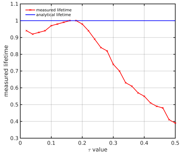
Figure 6. Measured lifetime of an eddy obtained by means of M_V (red line) versus the chosen \tau (analytical lifetime T_e = 1 (blue line), vortex strength 200).
