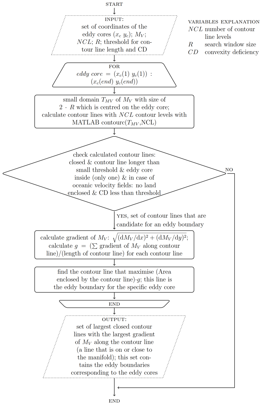
Figure S3. Schematic sketch of the eddy shape algorithm based on the combination of the Euler-Lagrangian descriptor M_V and the Lagrangian descriptor \mathcal{A}M_V .
