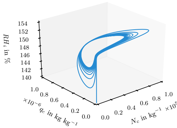
Figure 6. Limit cycle for state 2: orbit in phase space at T = 210\text{ K} , w = 0.02\text{ m s}^{-1} . Note that the solution starts “outside” of the limit cycle and approaches the limit cycle attractor asymptotically.
