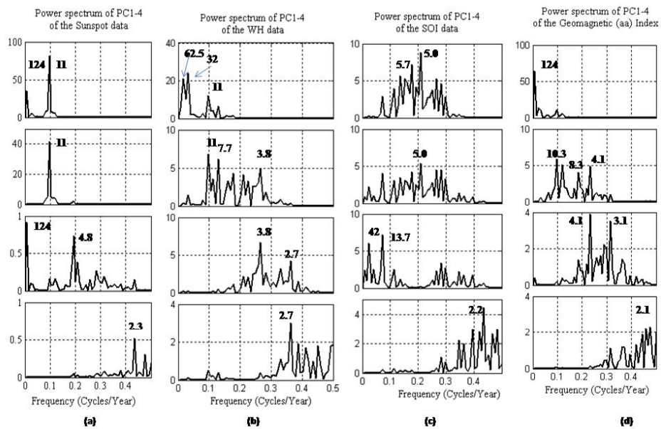
Fig. 3. Power spectra of the first four principal component (PCs) (PC1-4 shown in Fig. 2) for all the data sets with their significant periodicities at 124, 11, 4 and 2.8 years are indicated in bold
