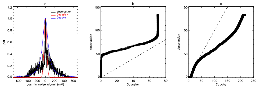
Fig. 3. Portrayals of the distribution of the stochastic component (described in the text) of the cosmic noise signal. Left: probability density function with fitted Gaussian (red) and Cauchy (blue) distributions superimposed (explained and discussed in the text). Centre: 480 Q-Q plot of the observed data versus Gaussian; right: Q-Q plot of the observed data versus Cauchy.
