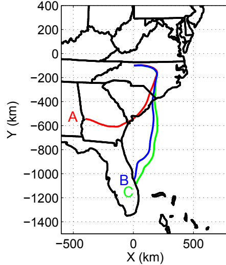
Figure 12. Three calculated trajectories of [hypothetical] collected samples. The red and blue trajectories correspond to the samples on either side of a LCS. The blue and green trajectories correspond to the samples on one side of the same LCS. Sampling times are 13:40, 14:00 and 14:10 UTC during the interrogation window (12:00 UTC 29 Sep to 12:00 UTC 30 Sep 2010) for the red, blue and the green particles, respectively. Source points of the collected particles are shown by A, B and C. Integration time for all three particles is T = 40 hr.
