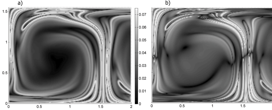
Figure 4. Forward FTLE field of an aperiodic Rayleigh-Bénard convection model. (a) The benchmark FTLE field at t_0 = 1 calculated by (6). (b) The approximated FTLE field calculated by (8), and \delta t = 0.1 time unit. A 4-th order Runge-Kutta integration scheme with constant integration time-step 0.01 and total integration time T = 75 units is implemented for both panels.
