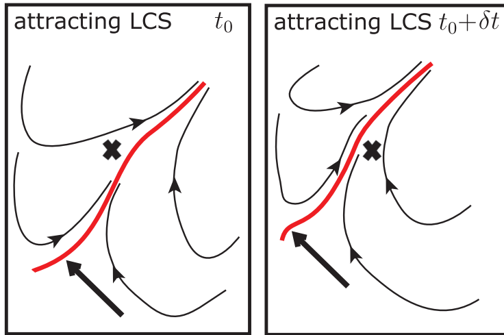
Figure 11. An attracting LCS feature (red) passes over the geographically fixed sampling location (indicated by a bold \times ). Black lines show trajectories of hypothetical particles that are absorbed to a moving attracting LCS. The bold arrow shows the general wind direction and the motion of the attracting LCS at the specified interval. Collected samples on either side of this attracting LCS feature come from two different regions.
