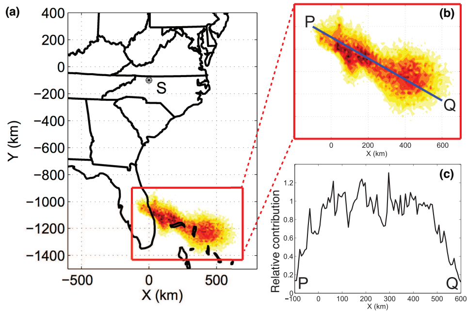
Figure 14. (a) The probabilistic equivalent of the source point of the [virtually] green particle in Fig. 12. The sampling point S is located at (0, -100) km with respect to our reference point and sampling time is 14:10 UTC 29 Sep 2010. (b) Details of the probabilistic source region which is composed of 5400 boxes, each 10\text{ km} \times 10\text{ km} . Color intensity shows the relative contribution of each source box. (c) \gamma , relative contribution of source boxes along the specified line PQ.
