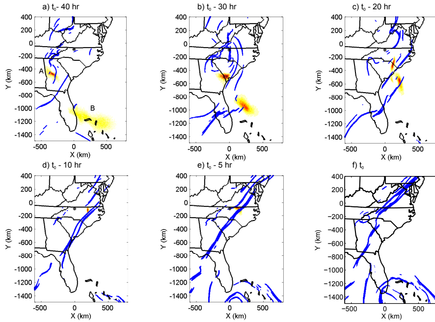
Figure 15. Sequence of the hyperbolic LCSs (blue) and two probabilistic source regions corresponding to two successive samples. Probabilistic regions “A” and “B” (panel (a)) correspond to the virtually red and blue particles in Fig. 12. These six panels correspond to 40, 30, 20, 10, 5 and 0 hours before collecting the corresponding samples at 13:40 and 14:00 UTC during the interrogation window.
