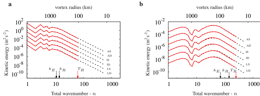
Figure 5. Scale by scale comparison of the benchmark simulation (dashed line) to the LES variants (red solid line). Kinetic energy spectra at the upper level of the: (a) atmosphere; and (b) ocean. The top pair of spectra exhibit the true energy, with subsequent pairs shifted down for clarity. Spectra are labelled with the associated subgrid parameterisation of anisotropic stochastic (AS), anisotropic deterministic (AD), isotropic stochastic (IS), isotropic deterministic (ID), scaling law stochastic (LS), or scaling law deterministic (LD). The truncation ( T_R ), Rossby ( k_R ) and energy containing ( k_E ) wavenumbers are labelled on the horizontal axis.
