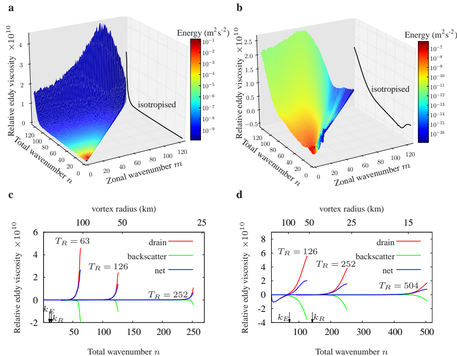
Figure 3. Real component of the upper diagonal subgrid eddy viscosities. Anisotropic drain eddy viscosity at T_R = 126 for the: (a) atmosphere, divided by the kinematic viscosity of air ( 10^{-5} \text{ m}^2 \text{ s}^{-1} ); and (b) ocean, divided by the kinematic viscosity of sea water ( 10^{-6} \text{ m}^2 \text{ s}^{-1} ). Coloured surfaces depict kinetic energy of the fluctuations at the upper level, and the black lines are the isotropised ( m averaged) drain coefficients. Isotropic drain, backscatter, and net eddy viscosities labelled by T_R for the: (c) atmosphere; and (d) ocean; with Rossby wavenumber ( k_R ) and energy containing wavenumber ( k_E ) labelled on the horizontal axes.
