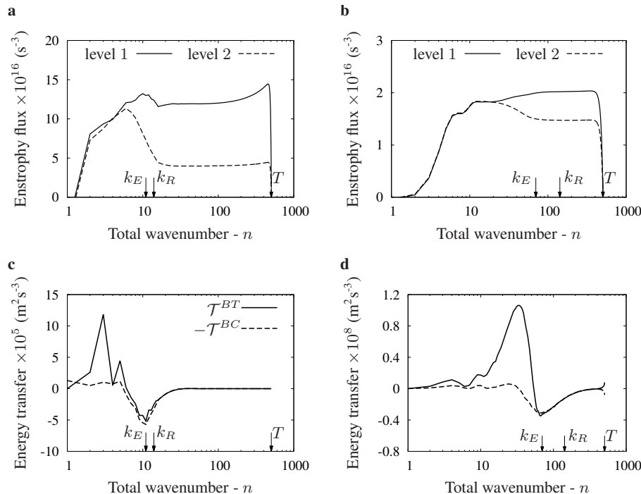
Figure 2. Spectral properties of the benchmark simulations. Potential enstrophy flux spectra on the upper vertical level (level 1) and lower level (level 2) for the: (a) atmosphere; and (b) ocean. Energy transferred into the barotropic mode ( \mathcal{T}^{BT} ) and out of the baroclinic mode ( -\mathcal{T}^{BC} ) for the: (c) atmosphere, with legend also applicable to (d) ; and (d) ocean. The energy containing scale wavenumber k_E , Rossby wavenumber k_R , and benchmark simulation truncation wavenumber T labelled on the n axis.
