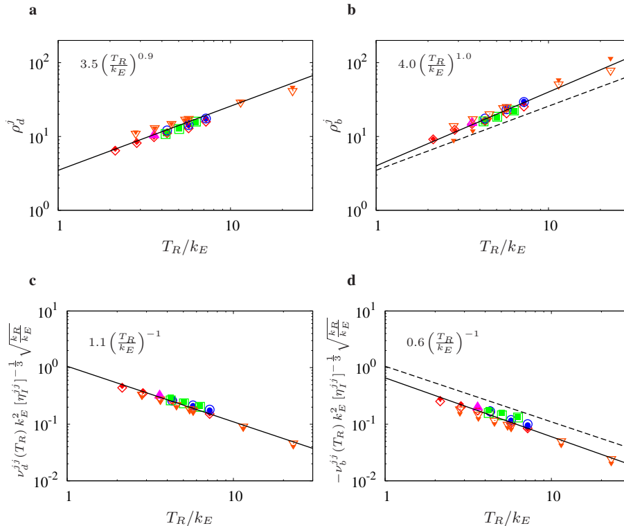
Figure 4. Scaling of the isotropic eddy viscosities. Slope of the: (a) drain eddy viscosity \rho_d^j ; and (b) backscatter eddy viscosity \rho_b^j . Magnitude of the: (c) drain eddy viscosity \nu_d^{jj}(T_R) ; and (d) negative backscatter eddy viscosity -\nu_b^{jj}(T_R) . The symbols correspond to the various cases as follows: red diamond, k_R = 142 , k_E = 70 ; blue circle, k_R = 284 , k_E = 70 ; green square, k_R = 142 , k_E \in (40, 50, 60) ; magenta upward pointing triangle, k_R \in (201, 246) , k_E = 70 ; orange downward pointing triangle, k_R = 14 , k_E = 11 (atmosphere). Filled symbols represent j = 1 and hollow symbols j = 2 .
