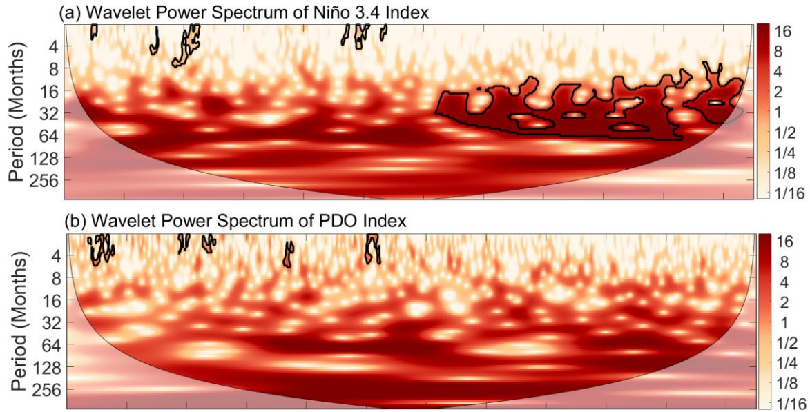
1 2 Figure 12. The application of the cumulative areawise test to the (a) Niño 3.4 index and (b) PDO 3 index. Contours enclose regions of 1% cumulative areawise significance.
