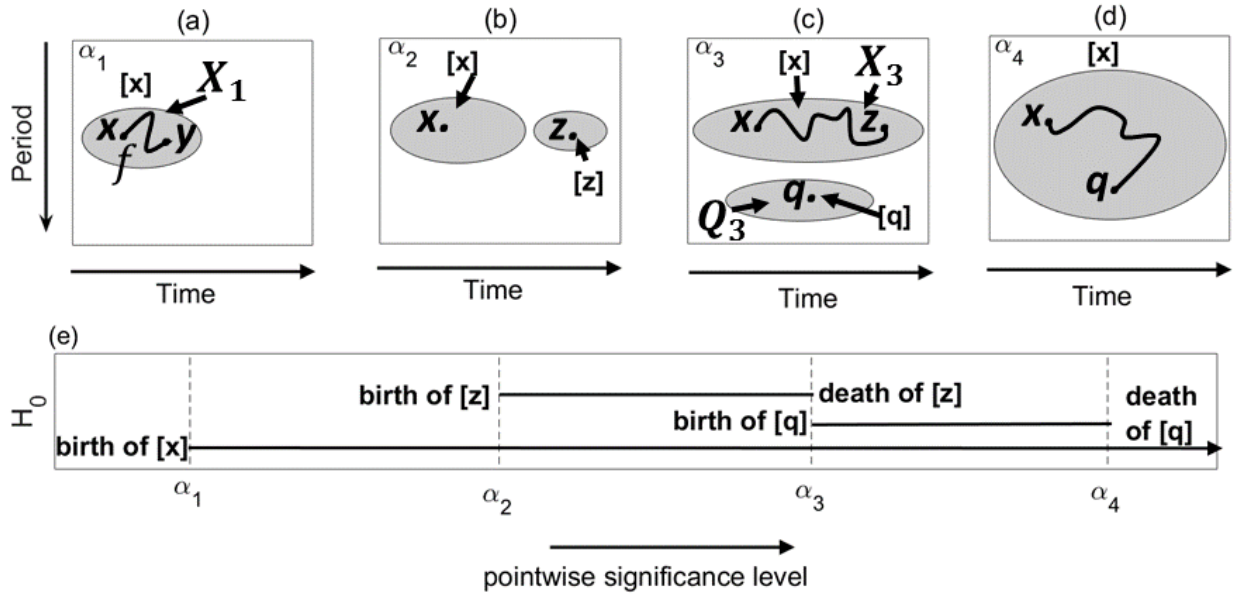
Figure 4. (a) - (d) The topological evolution of patches across four pointwise significance levels. (e) The barcode showing the birth and death of patches throughout the evolution process. Horizontal lines with arrows indicate those patches that never die.
