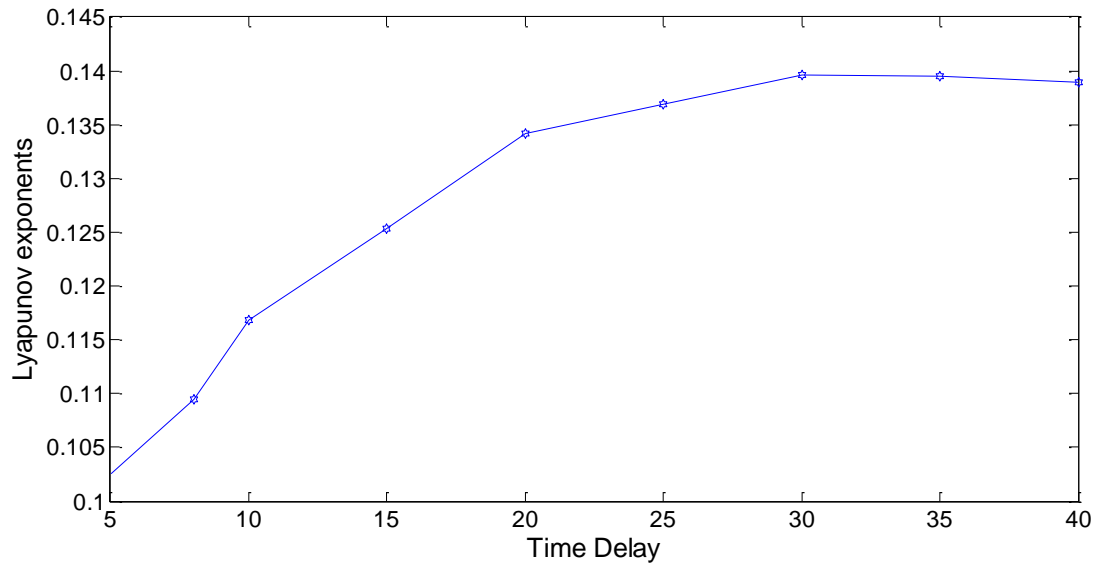
Fig 1 Different Lyapunov exponent computed for different time delay with a constant embedding dimension
