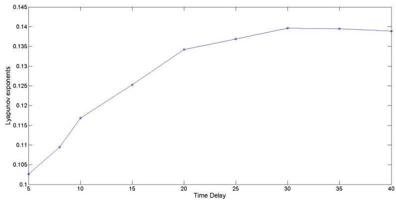
Fig. 1. Different Lyapunov exponents computed for different time delay with a constant embedding dimension
