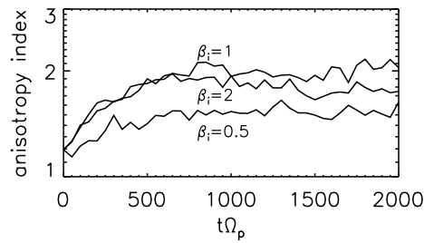
Figure 5. Anisotropy evolution for the data obtained by numerical simulation at the values of ion beta \beta_i = \{0.5, 1, 2\} .
