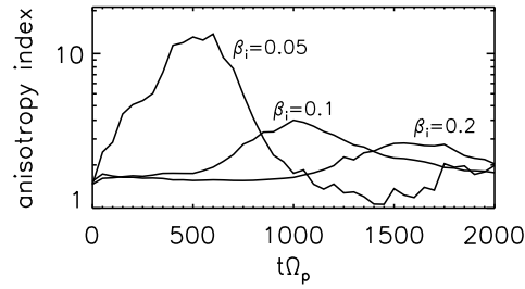
Figure 4. Anisotropy evolution for the data obtained by numerical simulation at the values of ion beta \beta_i = \{0.05, 0.1, 0.2\} .
