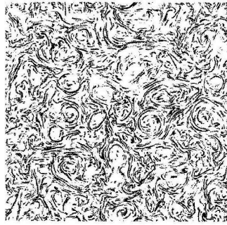
An initial turbulent vorticity field
