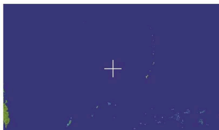
Small scale atmospheric turbulence over the ocean
