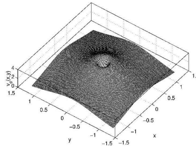
Asymptotic quasi-coherent structure
