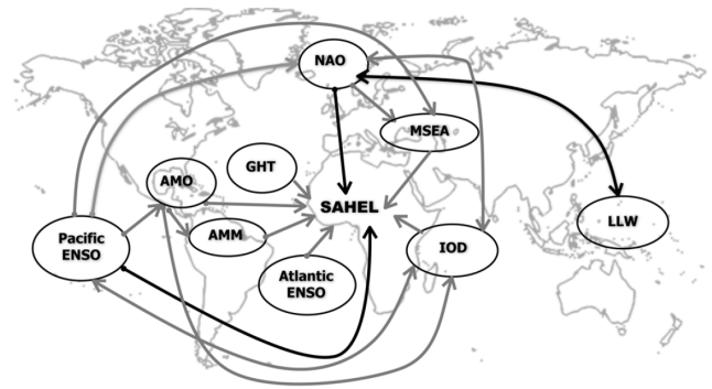
Fig. 1. Complex relationships between climate indices and Sahelian rainfall, with some direct and indirect relationships well defined in literature (light arrows) and others not fully understood (dark arrows)
