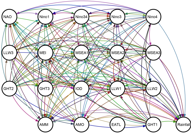
Fig. 8. Resulting combined network for coupling inciter EATL_8
