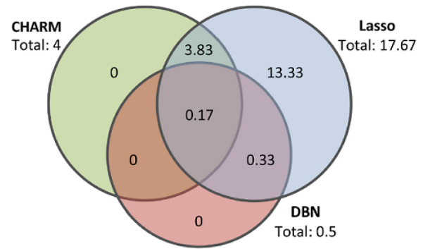
Fig. 10. Number of relationships found directly related to rainfall, averaged across coupling inciters
