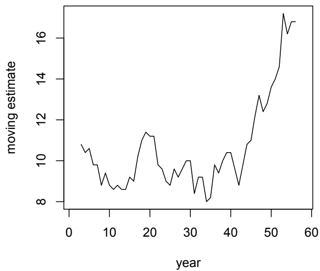
Fig. 3. A moving average estimate of the average number of hurricanes between the years 1951-2008.
