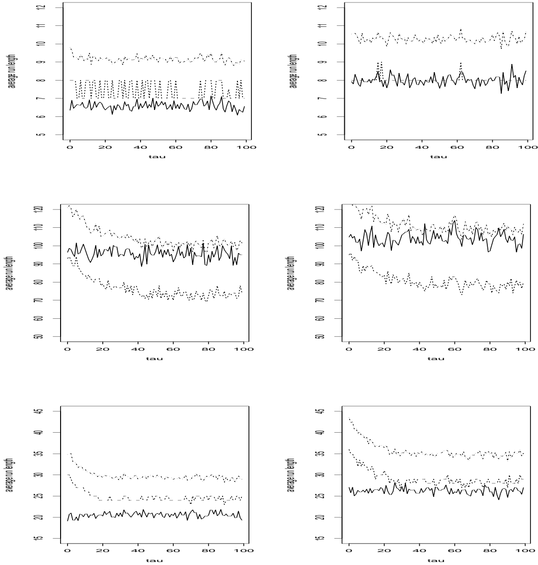
Fig. 1. Performance Comparison: Exponential Family CUSUM with Gaussian-CUSUM. Dotdash, dashed and solid line stand for mean, median and standard deviation. The top panel describes run length comparison from Binomial(15,0.95) to Binomial(15,0.90), the middle panel describes run length comparison from Poisson(3) to Poisson(3.1), the bottom panel describes run length comparison from Gamma(1,2) to Gamma(1.5,1.5). Due to length limitation of the graphs, we here do not include the MAX line.
