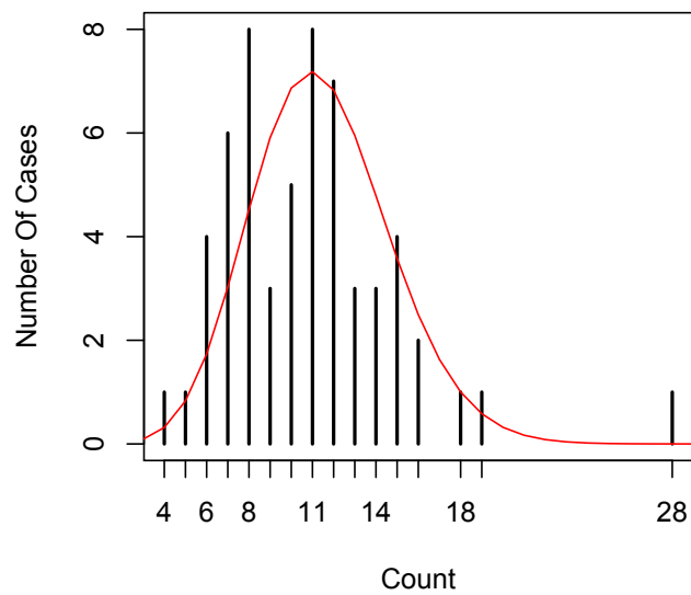
Fig. 2. The observed data and a Poisson fit for the number of hurricanes between the years 1951-2008.
