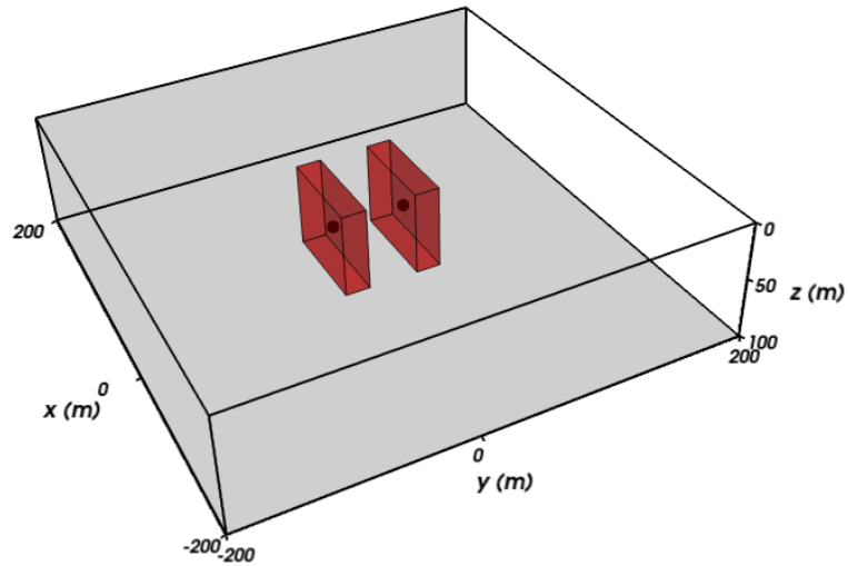
Fig. 8. Strong-interfering anomalies. Synthetic prisms (in red) with side lengths equal to 80 m, 20 m and 70 m along the x , y and z directions, respectively. Both prisms have a depth of the top at z = 10 m. The eastern prism has its centre at x_c = 0 m, y_c = -30 m and z_c = 45 m while western prism has its centre shifted 60 m in the positive y direction (pinpointed black dots).
