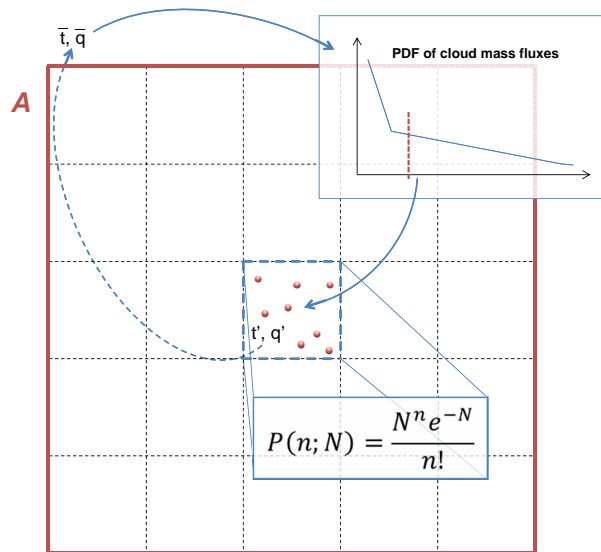
Figure 6. Schematic representation of the stochastic PC-2008 approach.
