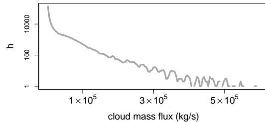
Figure 4. Semi-logarithmic plots of the cloud rate density distribution of cloud-base mass flux and the cloud failure rate function. These plots are corresponding to the RICO-140 simulation time frame of 6–12 h. The cloud rate density distribution is fitted using the mixdist R package (R Core Team, 2013), and the distribution shape parameter is set as equal for both distribution modes: k_1 = k_2 = k .
