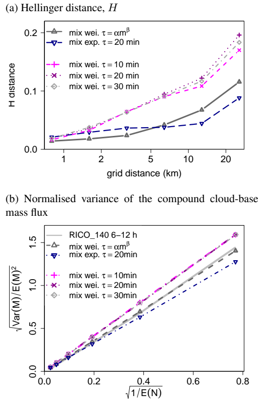
Figure 12. Comparison of the distribution pairs from the simulations using a constant and the mass-flux-dependent cloud lifetime.
