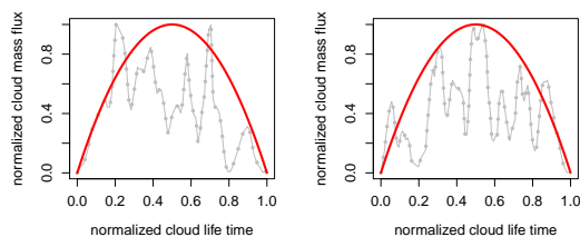
Figure 8. Idealised function for the cloud lifecycle (red) and the examples of individual cloud lifecycles (grey dots) from the LES RICO-140 case, after the cloud tracking.
