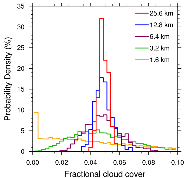
Figure 5. Histograms of the fractional cloud cover at the 700m height level for the different horizontal resolution of the LES coarse-graining.
