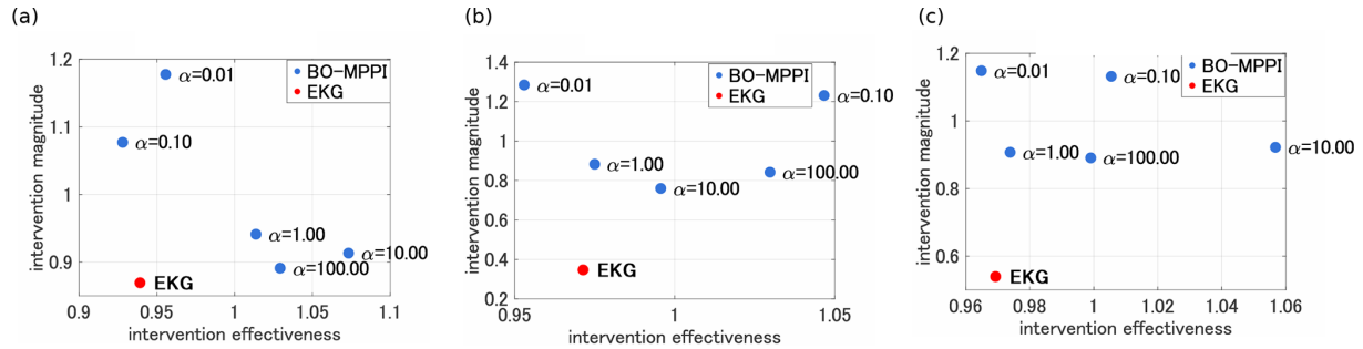
Figure 2. Comparison between BO-MPPI and EKG-MPPI for different values of \lambda : (a) \lambda = 0.1 , (b) \lambda = 1.0 , and (c) \lambda = 10 .
