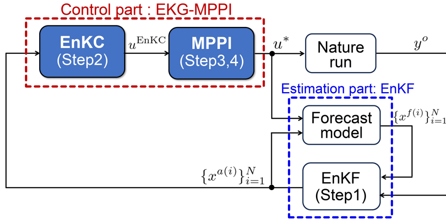
Figure 1. Block diagram of the proposed EKG-MPPI.
