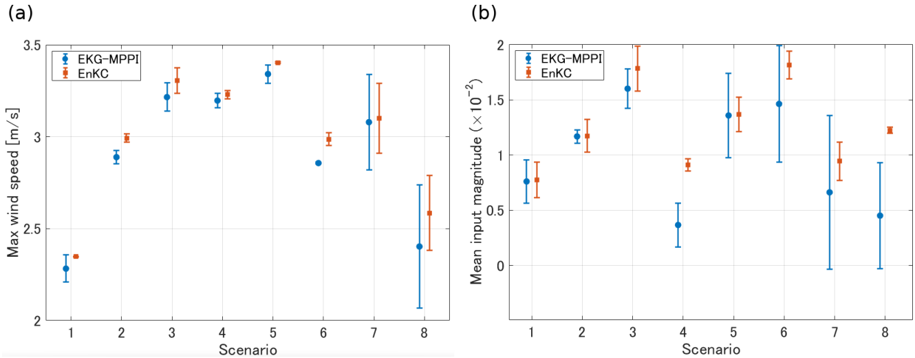
Figure 4. Mean and standard deviation of (a) the maximum wind speed and (b) the mean input magnitude for each scenario. Smaller values indicate better performance in terms of extreme-event suppression and control effort, respectively. The panels display raw values for each scenario rather than percentage differences.
