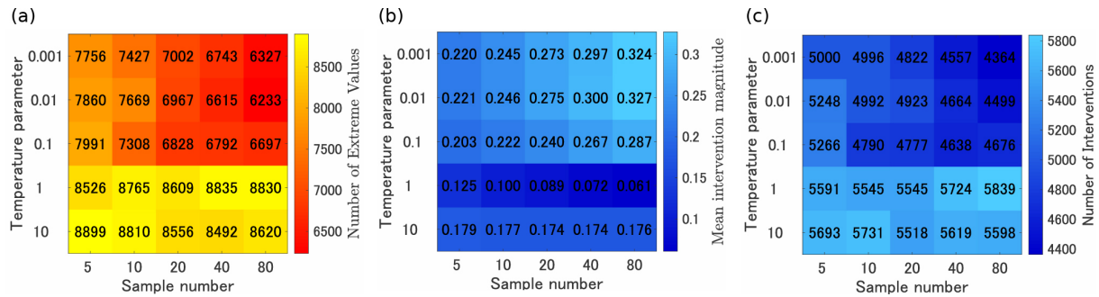
Figure 3. Hyperparameter configuration maps displaying the effects of varying \lambda and sample size on control outcomes: (a) number of threshold exceedances, (b) mean control-input magnitude, and (c) number of time steps at which control is applied.
