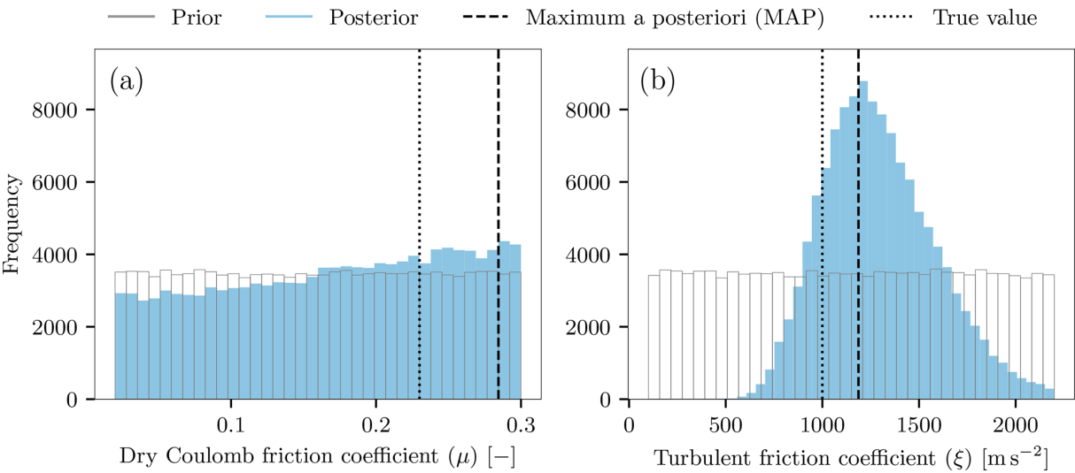
Figure 7. Posterior and prior distributions of (a) Dry Coulomb friction coefficient ( \mu ) and (b) Turbulent friction coefficient ( \xi ) based on calibration with maximum velocity ( U_{\text{max}} ) as observation. Maximum velocity conveyed more information about \xi during calibration, as reflected in the narrower posterior distribution.
