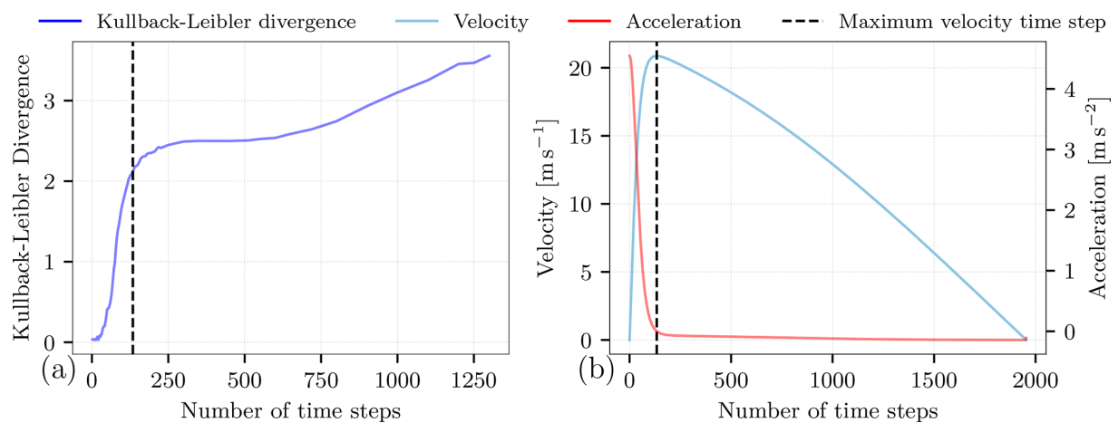
Figure 12. (a) Variation of Kullback-Leibler divergence of the posterior and prior distributions of turbulent friction coefficient \xi with velocity time steps. (b) Variation of velocity and acceleration with time steps.
