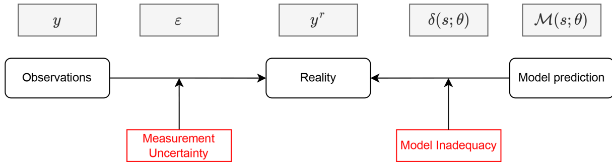
Figure 1. Statistical model connecting model predictions, reality, and observations. Adapted from Wu et al. (2018).
