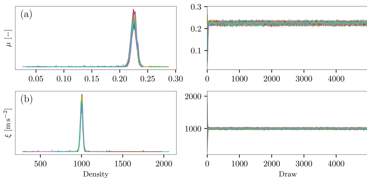
Figure B3. MCMC trace plots for (a) Dry Coulomb friction coefficient ( \mu ) and (b) Turbulent friction coefficient ( \xi ) based on calibration with velocity time series as observation. Each color represents an independent chain. Left panels show kernel density estimates of the marginal posterior distributions. Right panels show trace plots across iterations, demonstrating chain convergence and adequate mixing.
