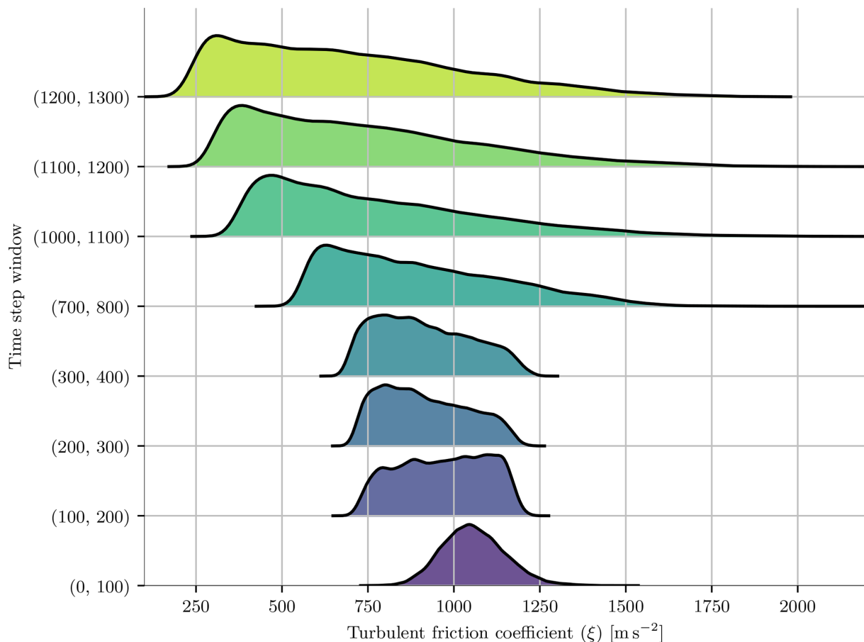
Figure C1. Posterior distributions of turbulent friction coefficient \xi calibrated with a fixed observation window of 100 time steps, with varying onset time. Initial time steps provide the highest information gain.
