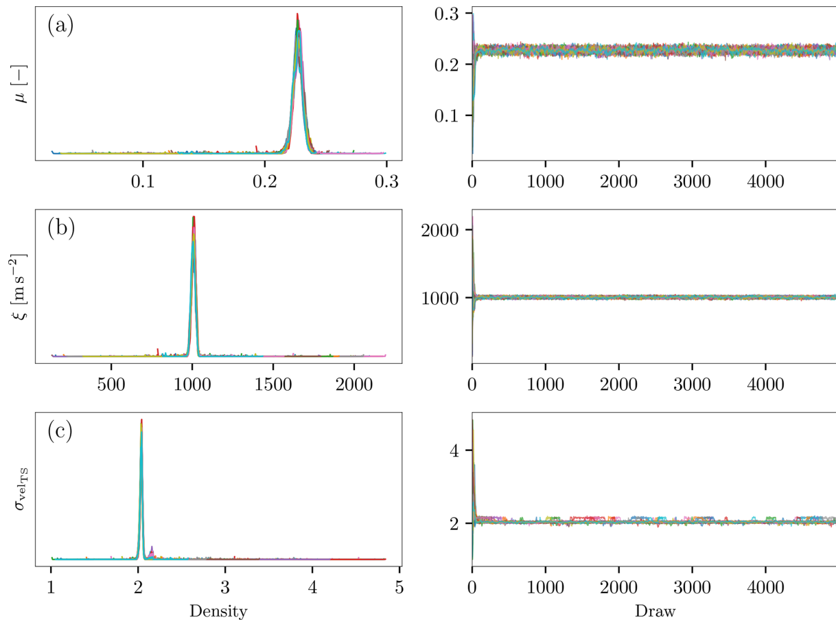
Figure B5. MCMC trace plots for (a) Dry Coulomb friction coefficient ( \mu ) and (b) Turbulent friction coefficient ( \xi ) (c) Velocity discrepancy parameter ( \sigma_{\text{velTS}} ) based on calibration with velocity time series as observation. Each color represents an independent chain. Left panels show kernel density estimates of the marginal posterior distributions. Right panels show trace plots across iterations, demonstrating chain convergence and adequate mixing.
