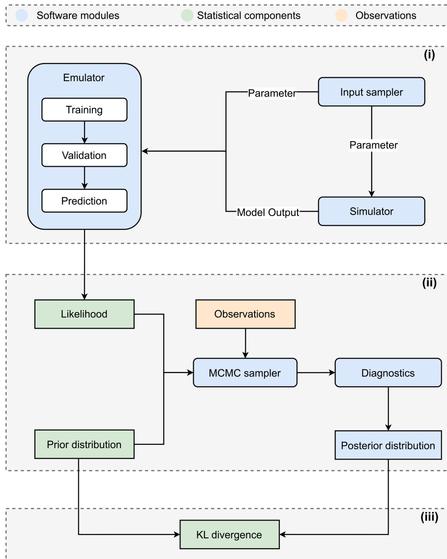
Figure 4. Overview of the Bayesian data selection workflow. The workflow consists of three key phases: (i) Surrogate Modeling, where a computationally efficient surrogate replaces the expensive forward model; (ii) Bayesian Parameter Calibration, where an MCMC sampler is used to infer the posterior distribution of the parameters; and (iii) Data Selection, where KL divergence quantifies the information gain from different observational data.
