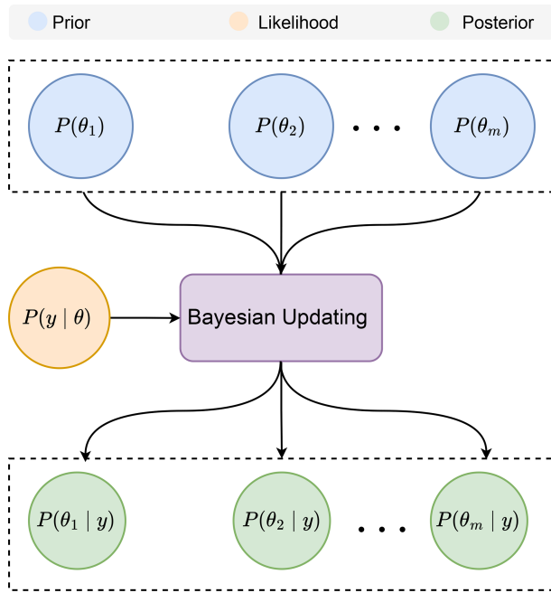
Figure 2. Schematic illustration of the Bayesian inference process. The likelihood function acts as the core driver of updating the prior distribution to posterior distribution based on observational data. The resulting posterior depends strongly on type and quality of the observation.
