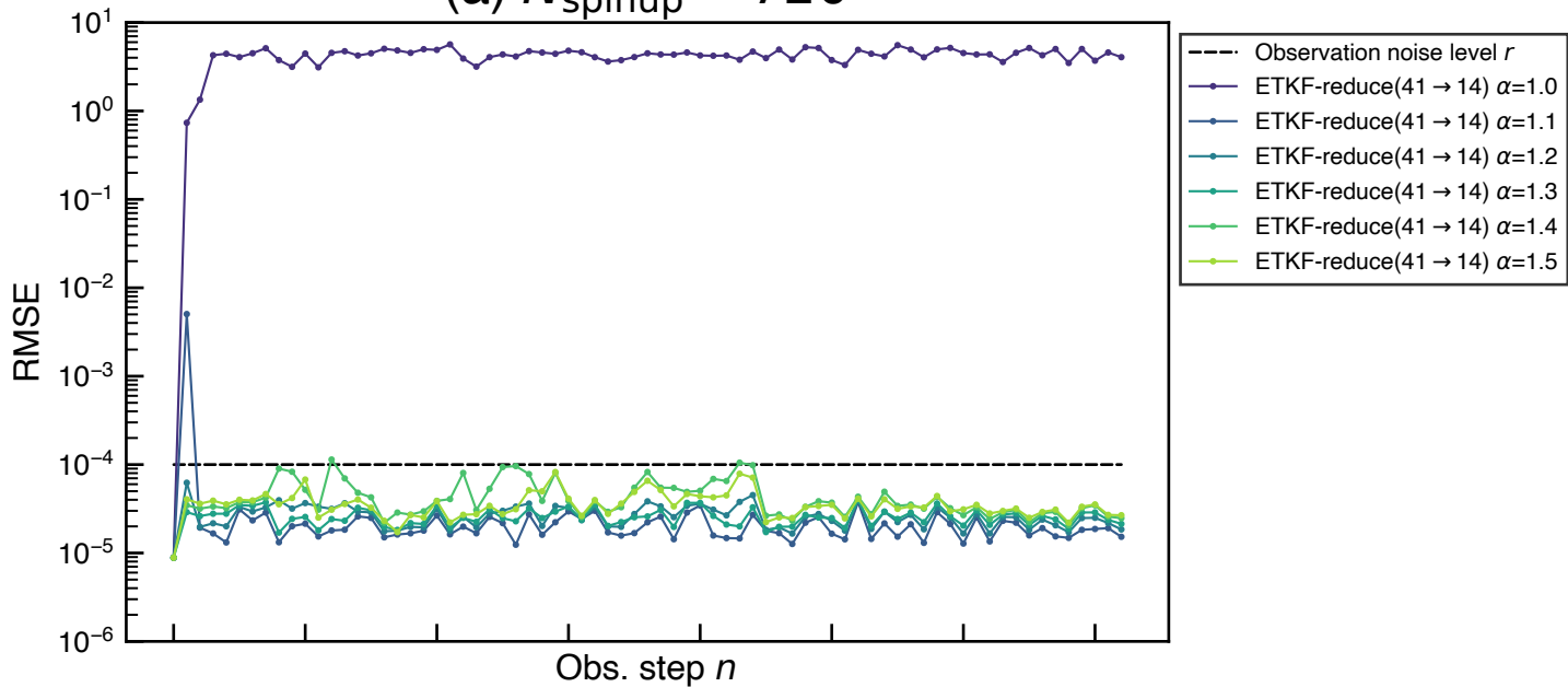
(a) N_{\text{spinup}} = 720
