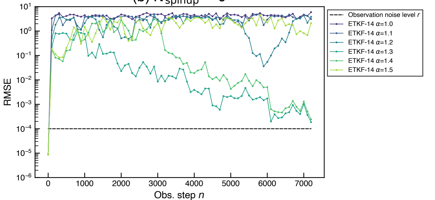
(b) N_{\text{spinup}} = 0
