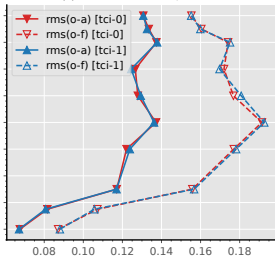
(c) statistics for TEMP, RH: rmse
