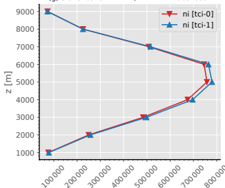
(g) statistics for RADAR, RADREFL: obs. count
