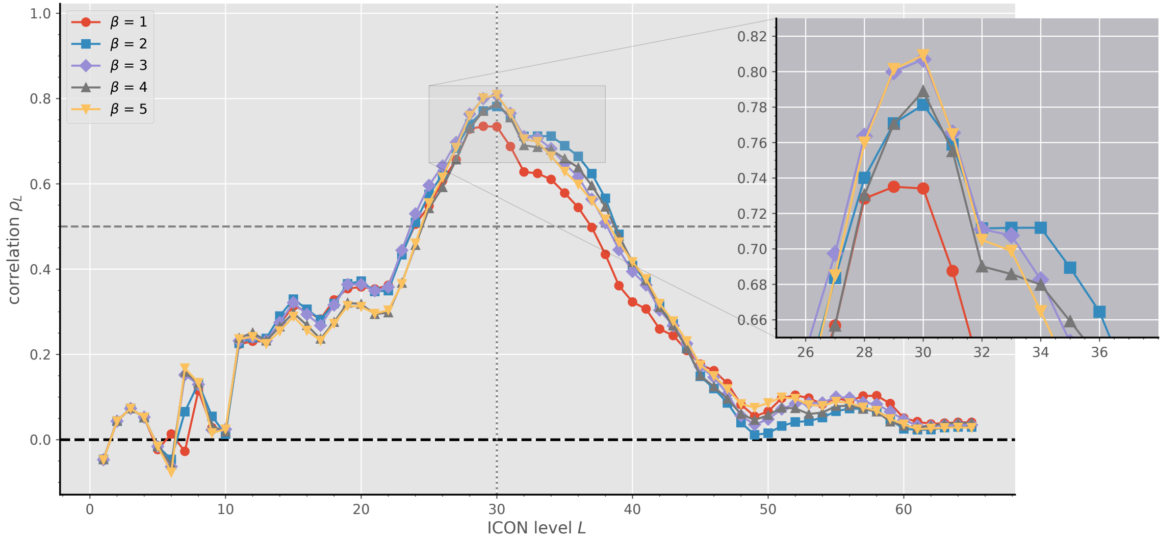
correlation of \delta Z with \delta q_v
