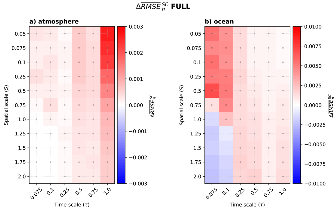
Figure 11. FULL experiment \overline{\Delta RMSE}_n^{SC} for (a) atmosphere and (b) ocean. The colour red (blue) indicates that the SC error is larger (smaller) than that of the WC experiments. Dotted area indicates \overline{\Delta RMSE}_n^{SC} \geq 0 , meaning that SCDA degrades over WCDA. Note that the colourbar for both components has different limits.
