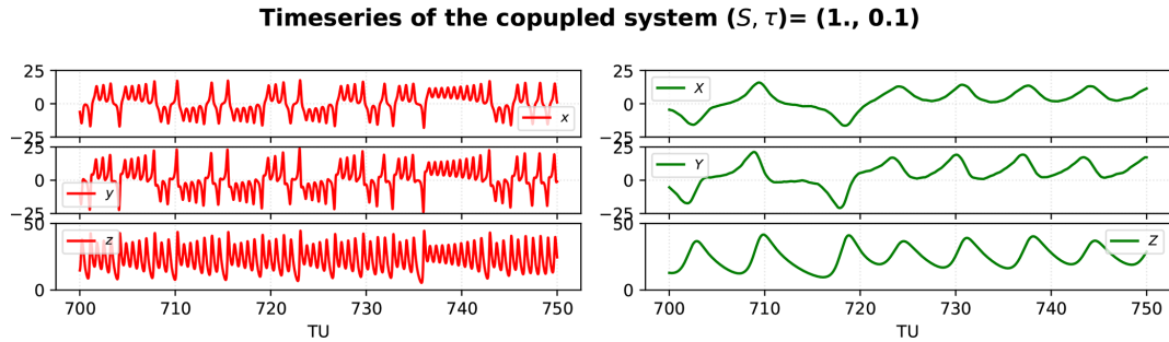
Figure 1. Time series of the atmospheric (left) and ocean (right) variables. The model uses here the configuration on Table 1, of the extratropical atmosphere-ocean system.
