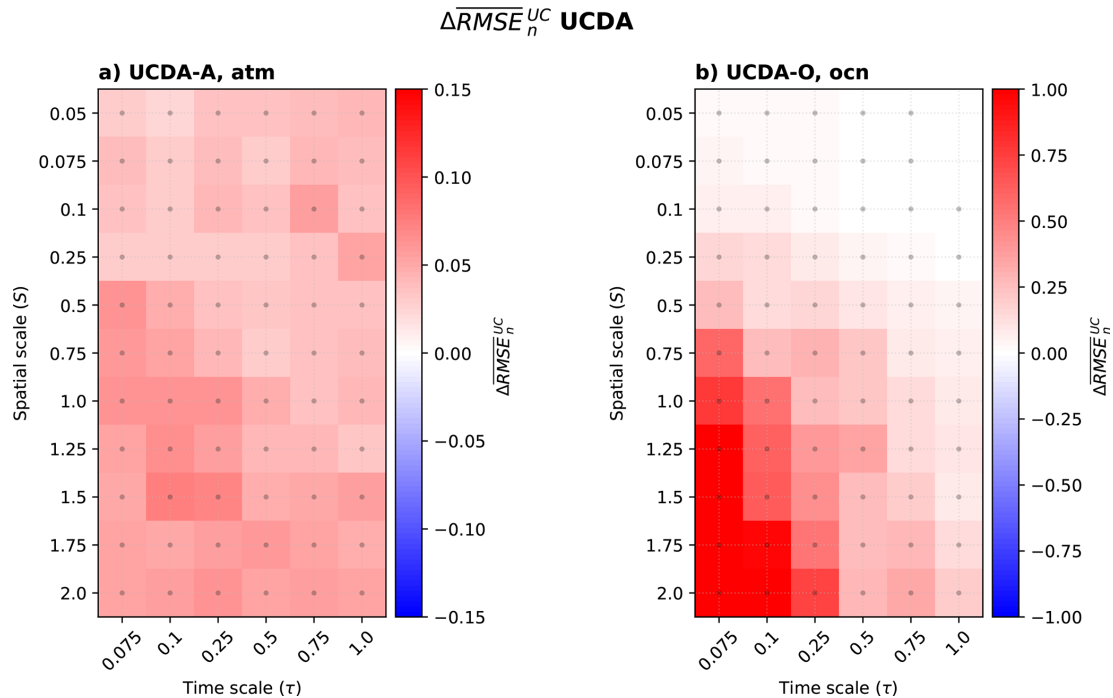
Figure 10. UCDA experiment \overline{\Delta RMSE}_n^{UC} for the uncoupled (a) atmosphere (UCDA-A) and (b) ocean (UCDA-O). The colour red (blue) indicates that the UCDA error is larger (smaller) than that of the WCDA experiments. Dotted area indicates \overline{\Delta RMSE}_n^{UC} \geq 0 , meaning that UCDA degrades over WCDA. Note that the colourbar for both components has different limits.
