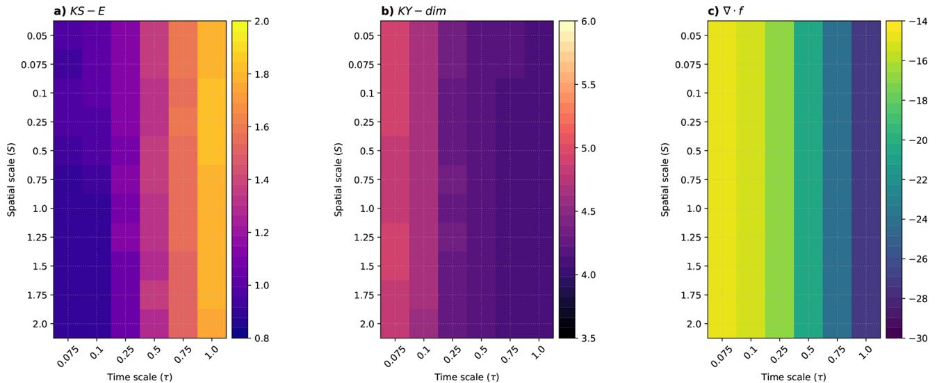
Figure 6. Stability analysis of the coupled system in dependence of the spatio-temporal parameters S and \tau (a) Kolmogorov–Sinai entropy KS-E , (b) Kaplan–York dimension KY-dim , and (c) divergence of the flow \nabla \cdot f . Note that each quantity has its own limits, and the colourbar is on a linear scale.
