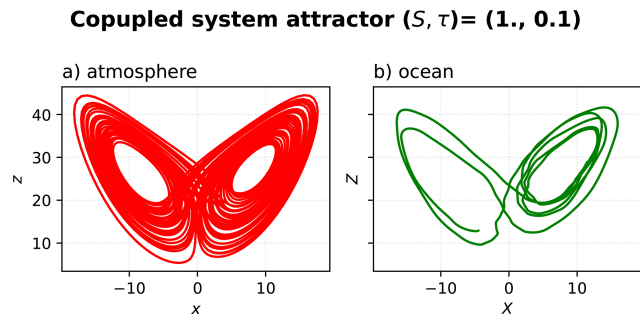
Figure 2. Standard configuration attractors of the extratropical atmosphere-ocean system during the 700–750 TU.
