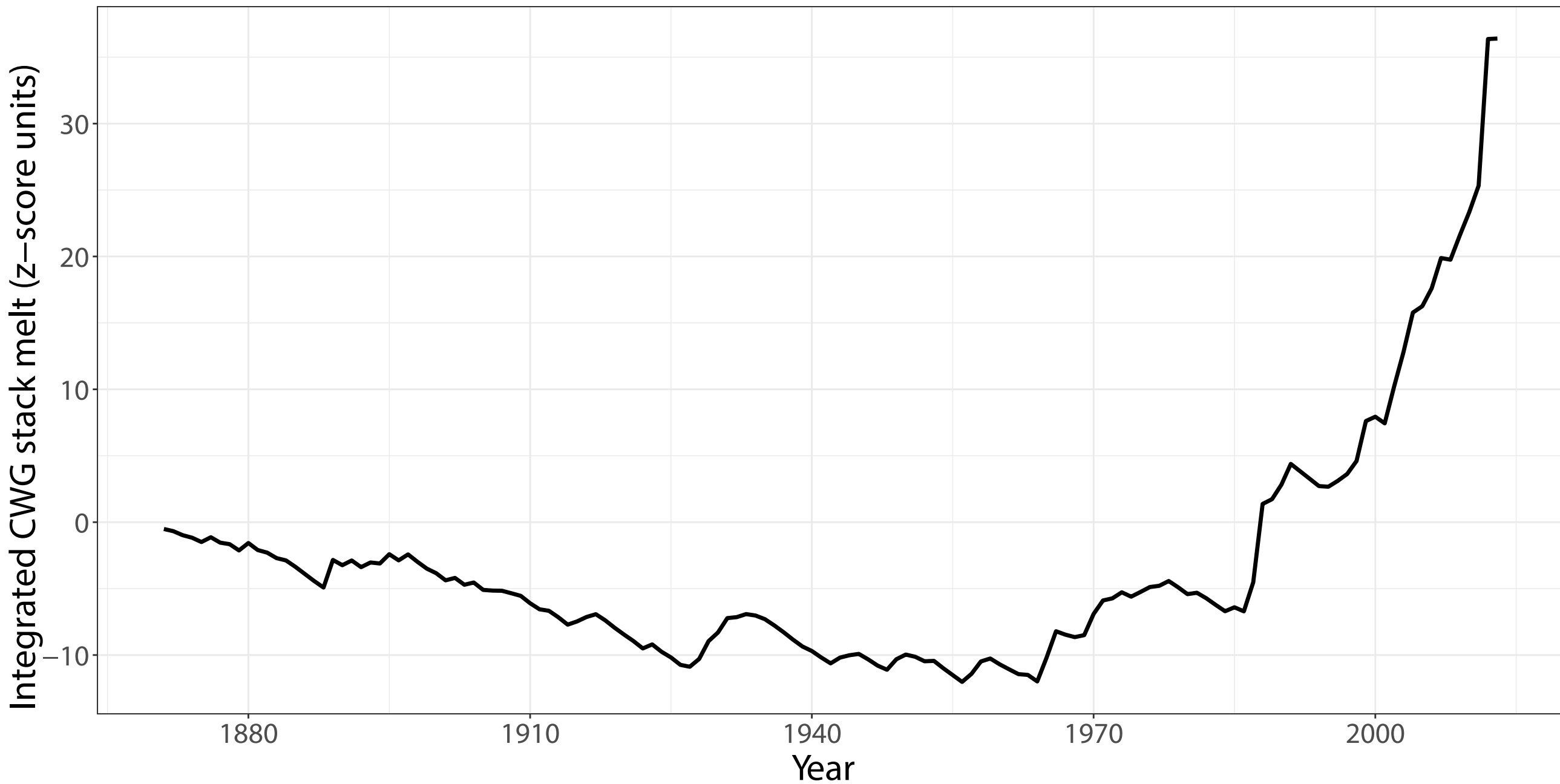
CWG surface melt Forcing
