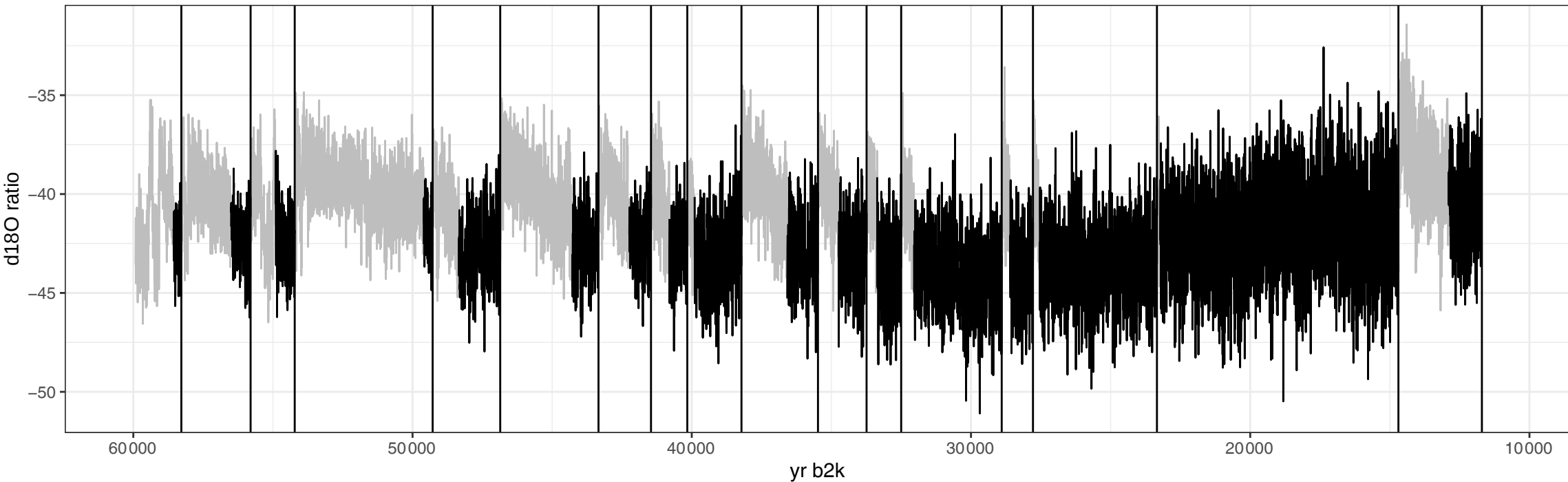
Dansgaard-Oeschger events in NGRIP d18O record
