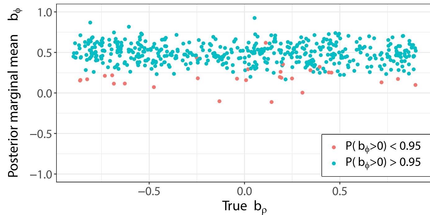
(c) Tipping process : b_\phi estimates vs true b_\rho
