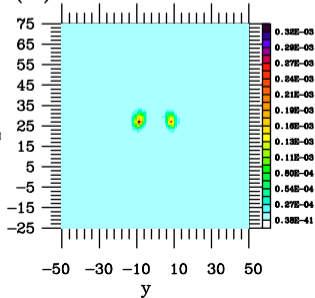
(e) t = 1.0
