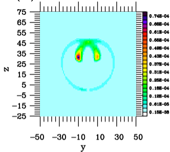
(h) t = 8.0
