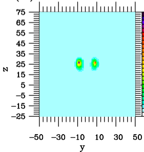
(f) t = 2.0
