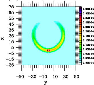
(g) t = 4.0
