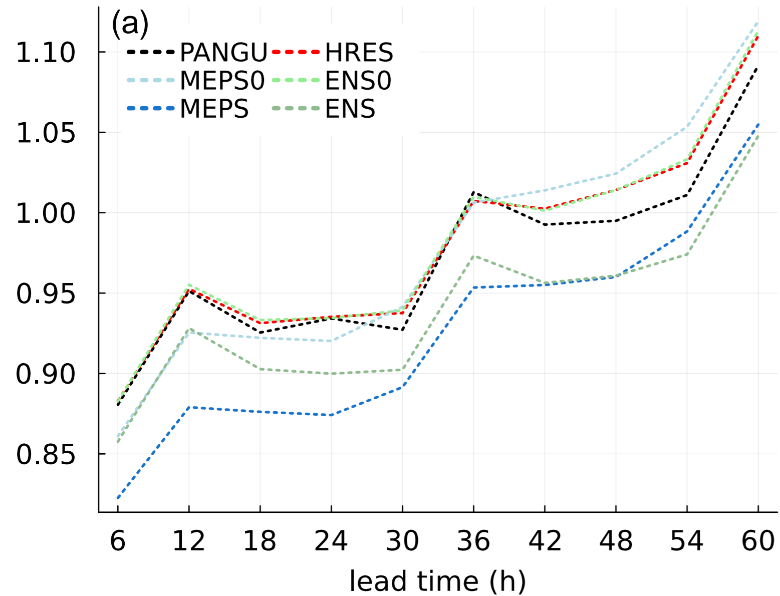
continuous ranked probability score ( \text{m s}^{-1} )
