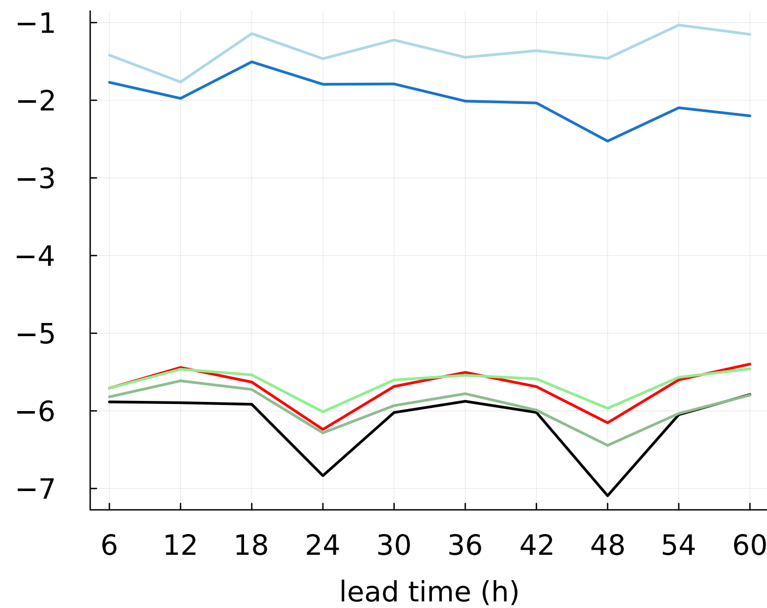
deviation in maxima ( \text{m s}^{-1} )
