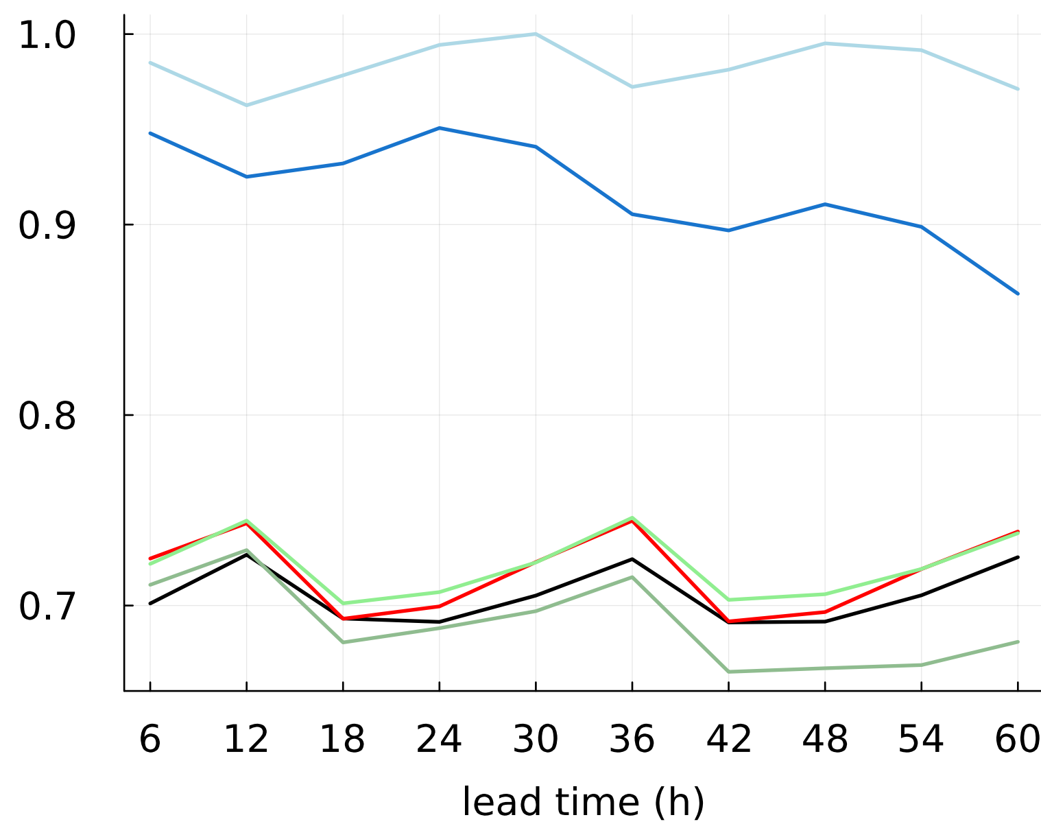
standard deviation ratio
