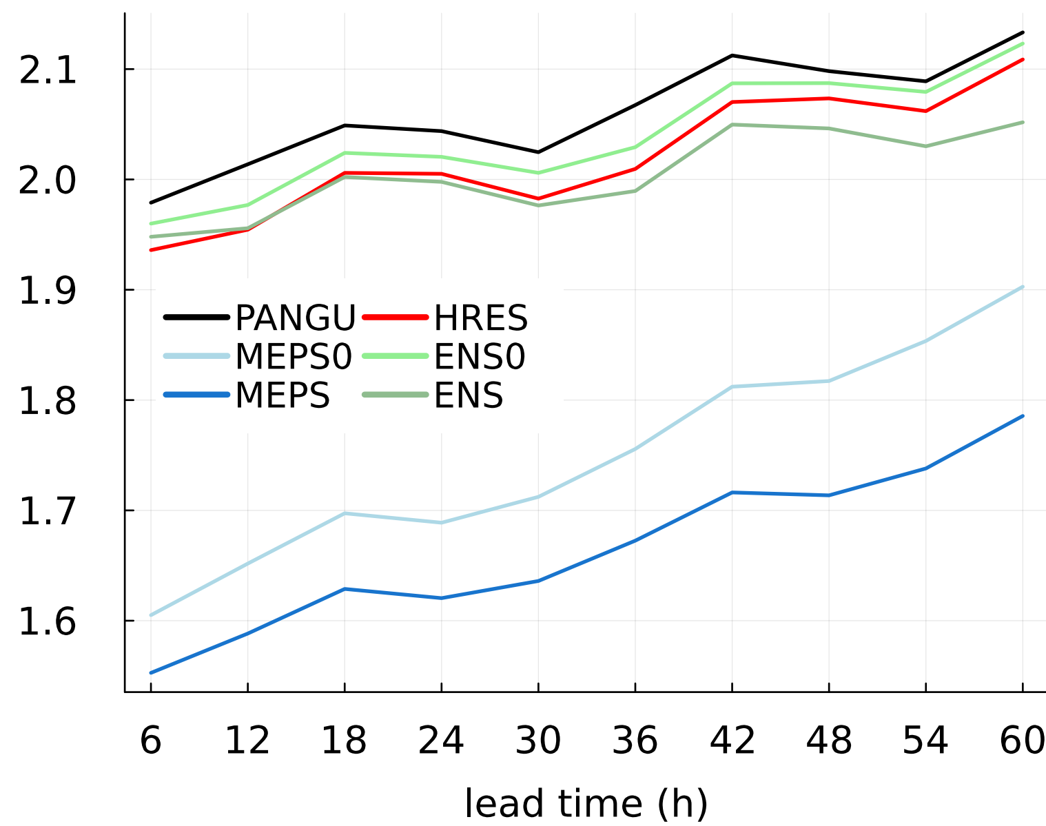
mean absolute error ( \text{m s}^{-1} )
