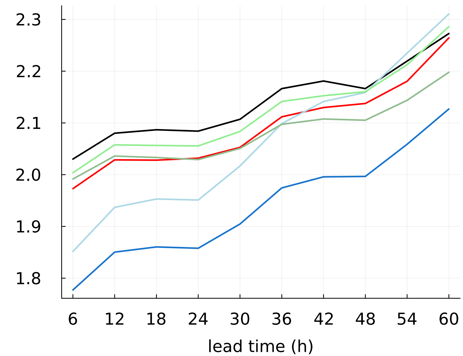
standard deviation of error ( \text{m s}^{-1} )
